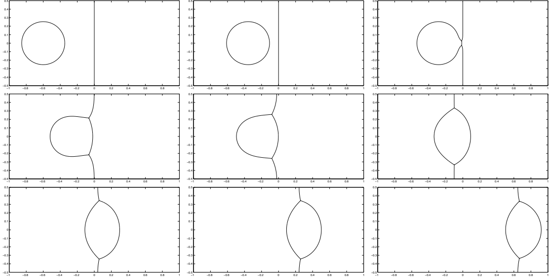
Figure 4: ( \gamma = \frac{1}{24\pi} , \alpha = 5\pi ) Solution (U_\varepsilon, V_\varepsilon) at times t = 0, 2 \times 10^{-3}, 2.6 \times 10^{-3}, 2.8 \times 10^{-3}, 3 \times 10^{-3}, 4 \times 10^{-3}, 6 \times 10^{-3}, 8 \times 10^{-3}, 0.012 .
