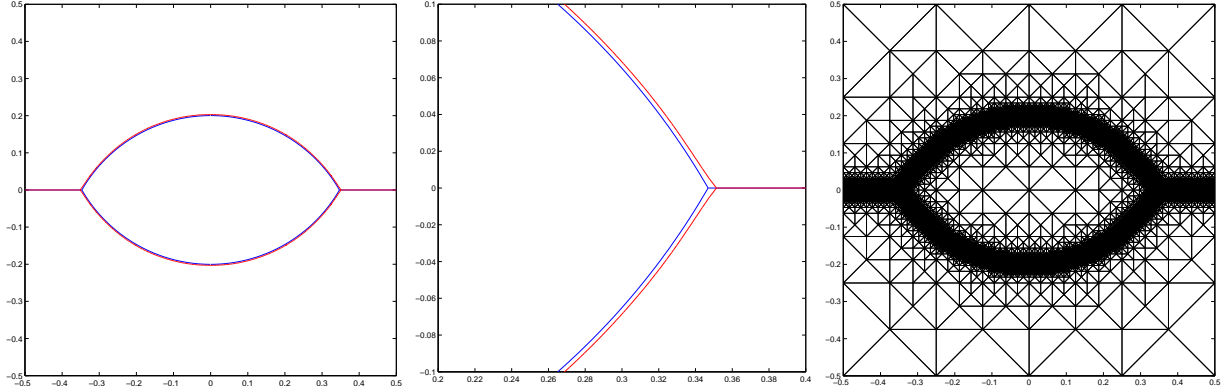
Figure 3: ( \gamma = \frac{1}{24\pi} , \alpha = 0 ) Comparison between computed solution (red) and true solution (blue). The final triangulation is shown on the right.
