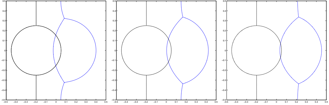
Figure 6: ( \alpha = 5\pi ) Solution (U_\varepsilon, V_\varepsilon) at times t = 0 , T = 4 \times 10^{-3} for \gamma = \frac{1}{12\pi} , \gamma = \frac{1}{24\pi} and \gamma = \frac{1}{48\pi} .
