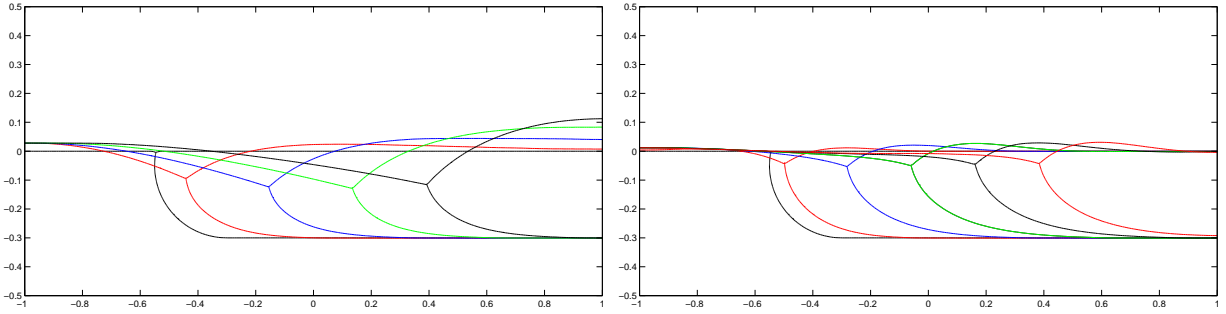
Figure 5: ( \gamma = \frac{1}{24\pi} , \alpha = 0 ) Solution (U_\varepsilon, V_\varepsilon) at times t = 0, 0.02, 0.06, 0.1, 0.14 for \beta = 1 (left); and t = 0, 2 \times 10^{-4}, 8 \times 10^{-4}, 1.4 \times 10^{-3}, 2 \times 10^{-3}, 2.6 \times 10^{-3} for \beta = \frac{1}{24\pi} (right).
