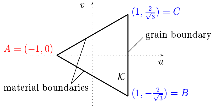
Figure 1: The (u, v) space \mathcal{K} = \triangle ABC . Here A represents the void phase, B grain I, and C grain II.
