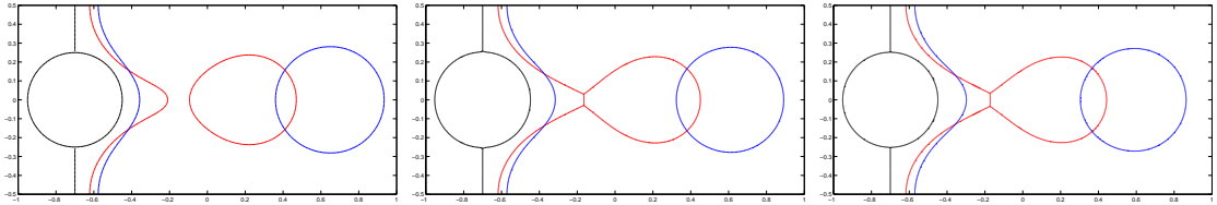
Figure 7: ( \alpha = 5\pi ) Solution (U_\varepsilon, V_\varepsilon) at times t = 0 , 0.04 , T = 0.056 for \gamma = \frac{1}{12\pi} , \gamma = \frac{1}{24\pi} and \gamma = \frac{1}{48\pi} .
