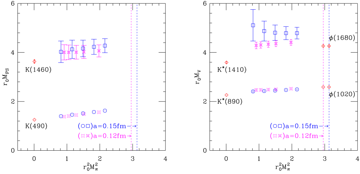
Figure 4: Ground- and excited-state meson masses vs M_\pi^2 for both lattice spacings. Both pseudoscalar and vector mesons are shown. One quark mass is fixed to the physical strange quark mass. All quantities are in units of the Sommer parameter r_0 . The diamonds represent the experimental points and the vertical lines mark the values of r_0^2 M_\pi^2 corresponding to the physical strange quark mass.
