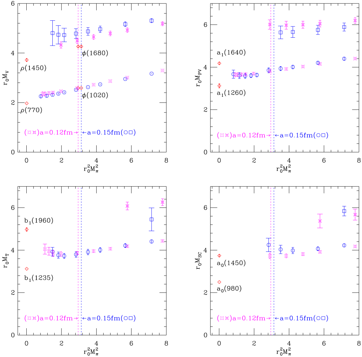
Figure 3: Ground- and excited-state meson masses vs M_\pi^2 for both lattice spacings. Vector, pseudoscalar, tensor, and scalar mesons appear. The quark masses are degenerate. All quantities are in units of the Sommer parameter r_0 . The diamonds represent the experimental points and the vertical lines mark the values of r_0^2 M_\pi^2 corresponding to the physical strange quark mass.
