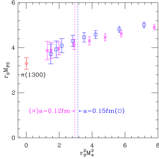
Figure 2: Excited-state pseudoscalar masses vs M_\pi^2 for both lattice spacings. The quark masses are degenerate. All quantities are in units of the Sommer parameter r_0 . The diamond represents the experimental point and the vertical lines mark the values of r_0^2 M_\pi^2 corresponding to the physical strange quark mass.
