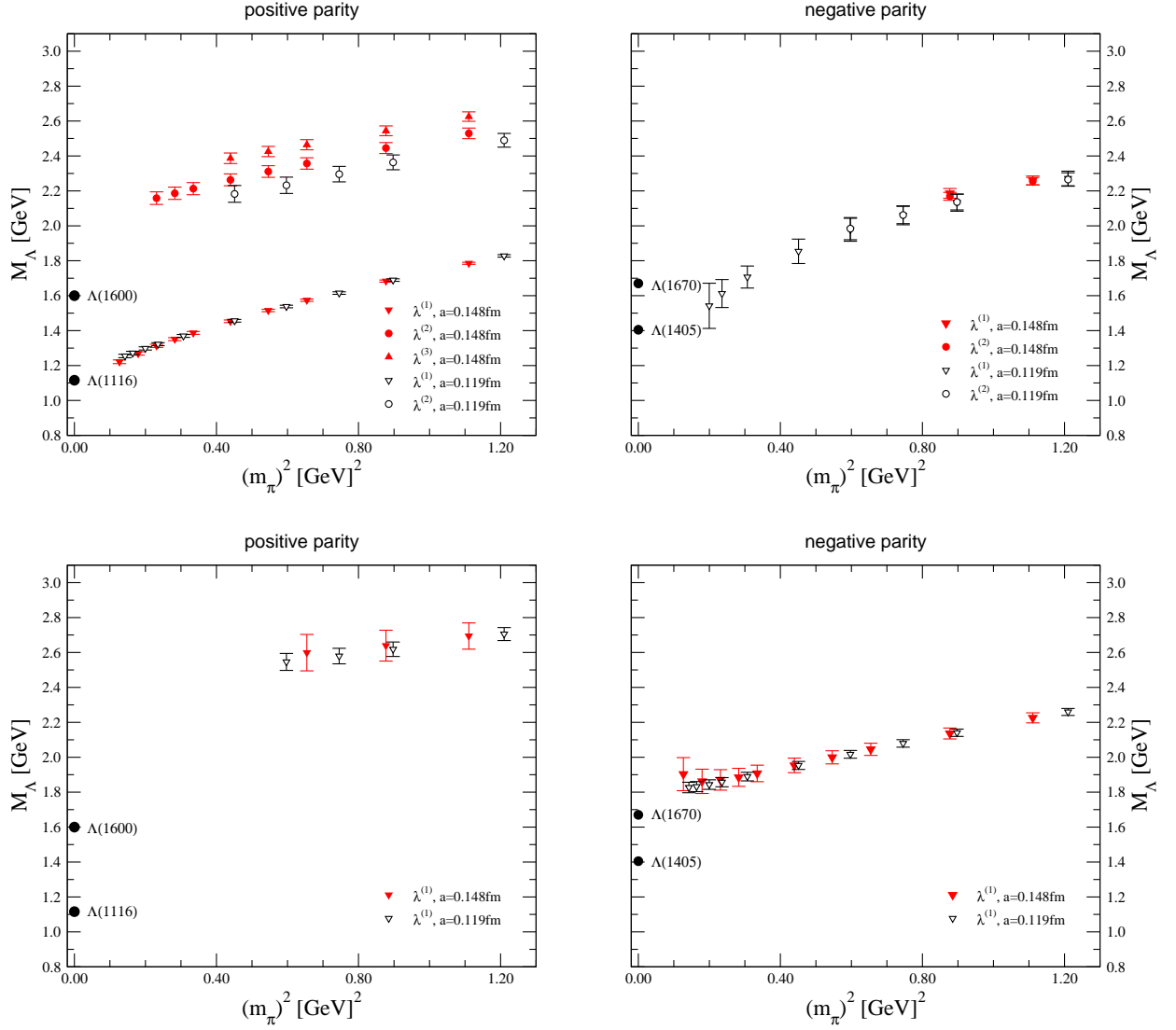
FIG. 6: Ground and excited state masses obtained from our \Lambda octet (upper plots) and \Lambda singlet (lower plots) interpolators.
