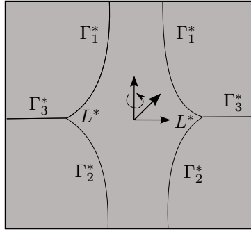
Figure 2: Example with specific geometry
