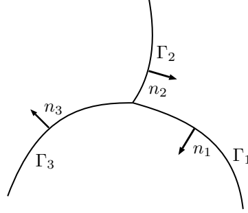
Figure 1: The choice of the normals.
