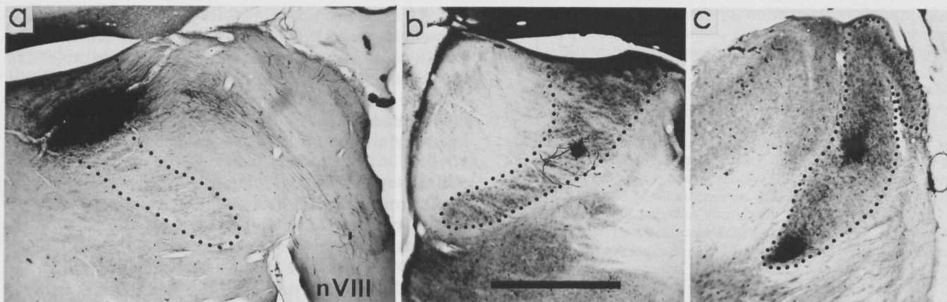
Fig. 2a–c. Photomicrographs of representative examples of injection sites, which led to peripherally-labelled neurones in the cochlear wholemount. Each panel shows part of a frontal brainstem section, with the cochlear nucleus outlined by a dotted border. Dorsal is always to the top, the midline to the left in a , to the right in b and c . Scale bar in b is 1 mm and applies to all 3 micrographs. a One
