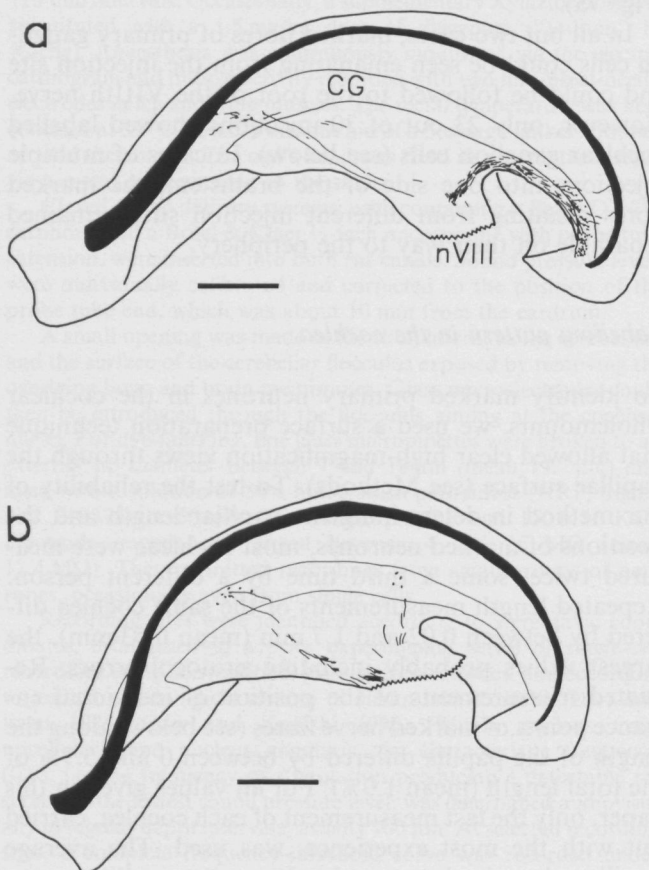
Fig. 3a, b. Schematic drawings of two cochlear wholemounts, as seen at low magnification. Apical is to the left, basal to the right, the cut end of the VIIIth nerve (nVIII) is indicated by a saw-toothed line. The basilar papilla is drawn as a solid black band, and the outline of the cochlear ganglion (CG) is indicated by thin lines. Scale bar 1 mm. Two groups of stained primary neurones can be distinguished in each case, in a their CFs were 9.6 kHz (for the group at the basal end) and 3.36 kHz, in b the CFs were 8.4 kHz and 5.3 kHz
