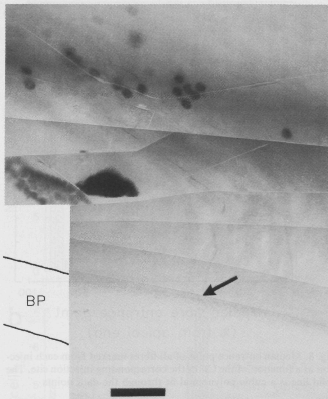
Fig. 5. Videomontage of a wholemout view of a group of labelled ganglion cells (at the top) with one marked fibre followed to its entrance point into the basilar papilla ( arrow ). The basilar papilla is not clearly discernable due to overexposure, therefore its neural and abneural borders are indicated on the left of the picture (BP = basilar papilla). Scale bar 100 \mu m
