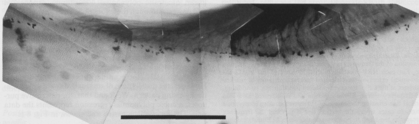
Fig. 6. Videomontage of a wholemout view onto the most apical 2 mm of papillar surface. Apical is to the left, neural to the top; scale bar 0.5 mm. Numerous labelled fibres can be seen entering the
