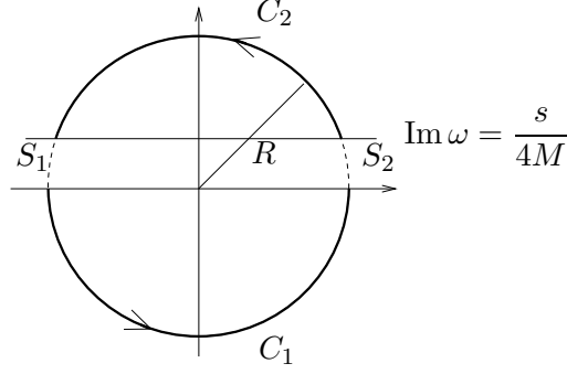
Figure 1: The contour C_R = C_1 \cup C_2 .
