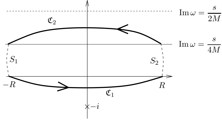
Figure 2: The contour \mathfrak{C}_R = \mathfrak{C}_1 \cup \mathfrak{C}_2 .
