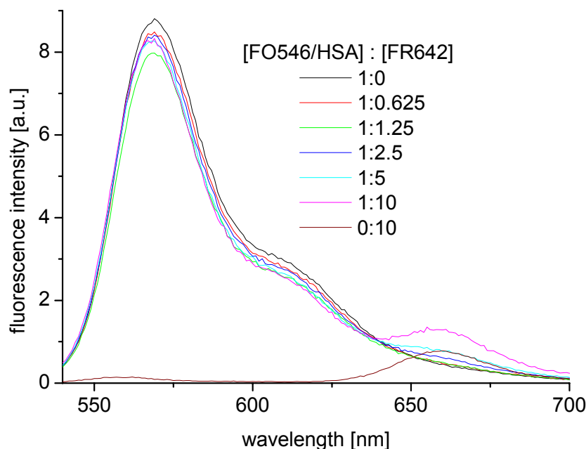
Figure 3.3. Fluorescence spectra of FO546/HSA (DPR = 2.1) of constant concentration titrated with free FR642 ( \lambda_{\text{exc}} = 520 nm). [\text{HSA}] = 1.0 \cdot 10^{-7} mol/L.
