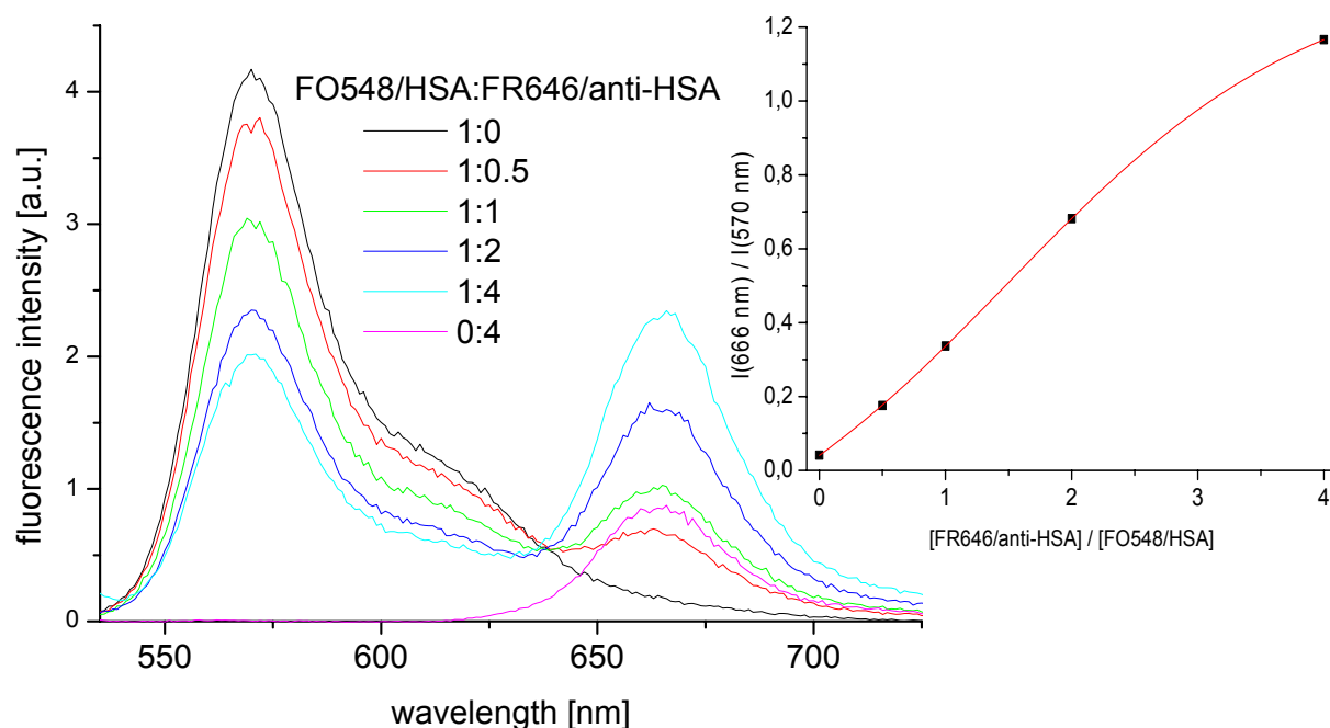
Figure 3.7. Energy transfer study in which FO545/HSA (DPR = 3.6) of constant concentration was titrated with FR646/anti-HSA (DPR = 1.5) ( \lambda_{\text{exc}} = 520 nm). [\text{HSA}] = 2.0 \cdot 10^{-8} mol/L.
