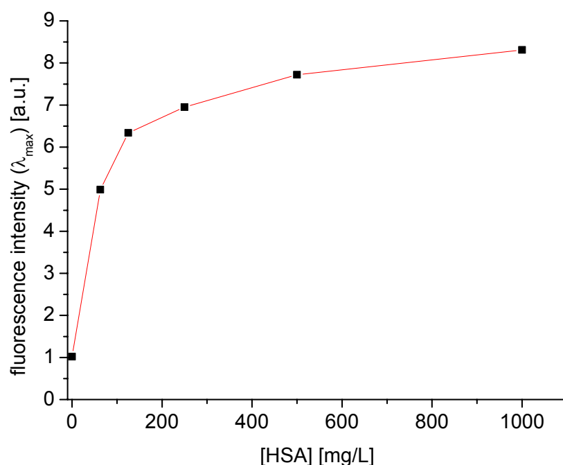
Figure 2.20. Plot of the fluorescence intensities of FR662 (free dye) at the emission maximum versus the concentration of added HSA. [\text{FR662}] = 6.8 \cdot 10^{-7} \text{ mol/L} . \lambda_{\text{exc}} = 640 \text{ nm} .
