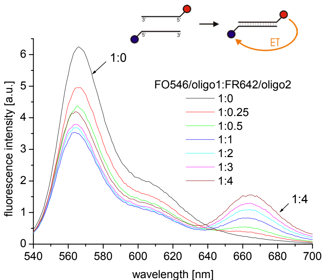
Figure 3.20. Energy transfer study in which FO546/oligo1 of constant concentration ( [\text{FO546/oligo1}] = 1.0 \cdot 10^{-7} \text{ mol/L} ) was titrated with FR642/oligo2 ( \lambda_{\text{exc}} = 530 \text{ nm} ).
