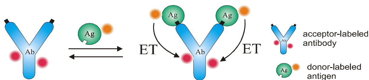
Figure 3.1. Scheme for energy transfer on the system HSA/anti-HSA
