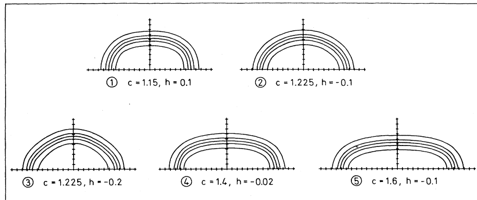
FIG. VII-8. Equipotential lines for some shapes in the \{c, h\} parametrization. The equipotential lines refer to the energies 0.1 V_0, 0.3 V_0, 0.5 V_0, 0.7 V_0 , and 0.9 V_0 , where V_0 is the well depth in the center. Each division on the axis represents 1 F. The spherical radius is taken equal to 7 F.
