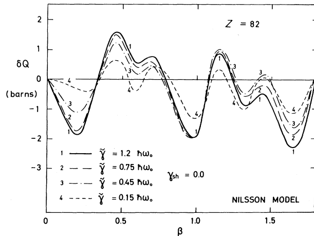
FIG. IV-7. The quadrupole moment \delta Q of the spatial density fluctuations, calculated with the Nilsson model ( Z=82 ) for different values of the smearing parameter \tilde{\gamma} ( \gamma_{sh}=0 ). Starting from the smallest values of \tilde{\gamma} (lines 4 and 3), the full value of \delta Q is essentially reached for \tilde{\gamma}=0.75\hbar\omega_0 .
