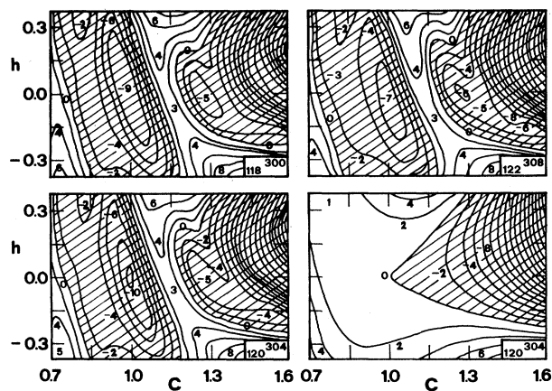
FIG. A-4. Same as Fig. A-3 for some other combinations of proton and neutron numbers. The lower map at the right-hand side shows, as an illustration, the LDM energy alone for the hypothetical ^{304}_{120} .
