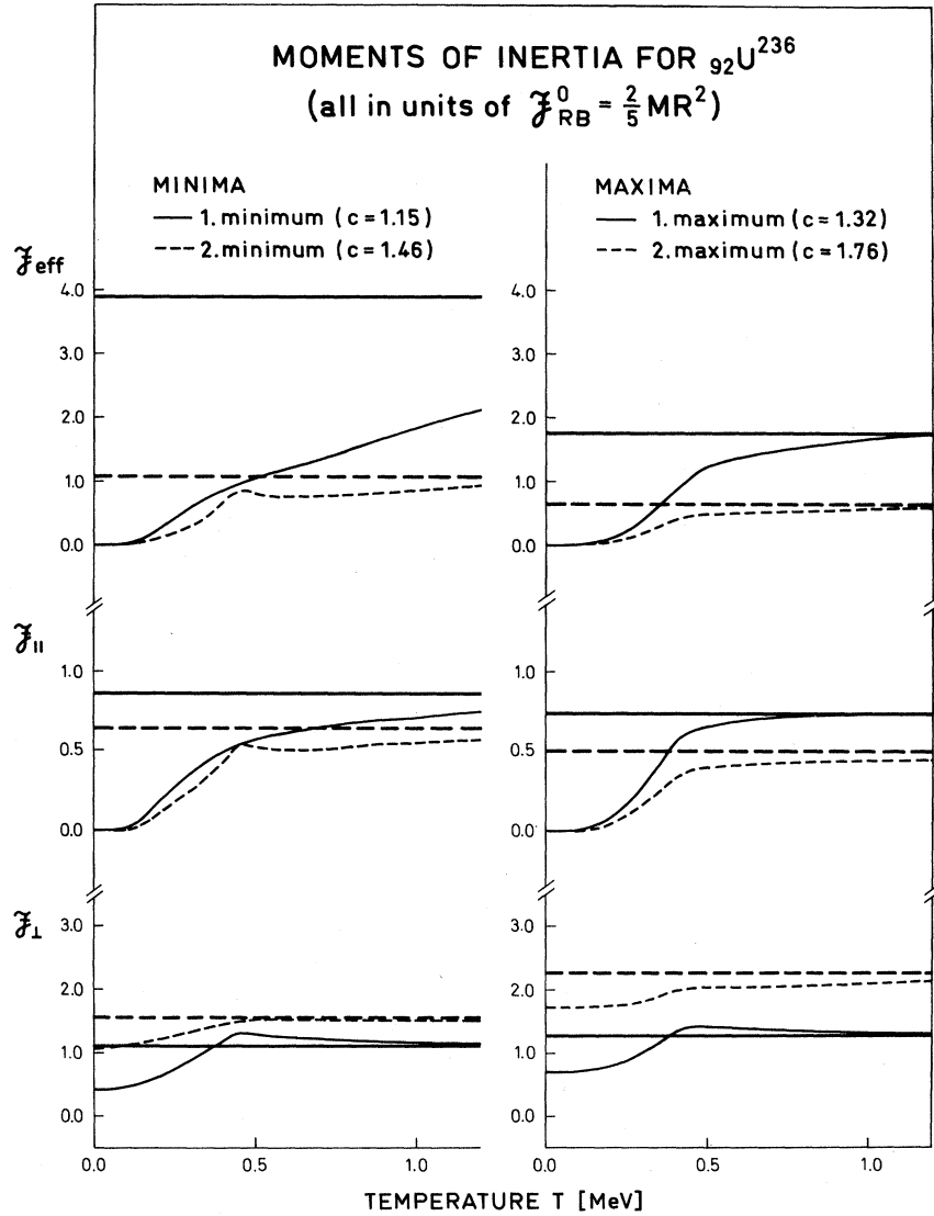
FIG. IX-15. The moments of inertia \mathcal{J}_{\text{eff}} , \mathcal{J}_{||} , and \mathcal{J}_{\perp} for ^{236}\text{U} , evaluated in the Woods-Saxon model (WS), are shown as a function of the nuclear temperature for the deformations at the ground state ( c=1.15 ), the second minimum ( c=1.46 ), the first barrier ( c=1.32 ), and the second barrier ( c=1.76 ). All the moments of inertia are expressed in units of the rigid-body value for a sphere, \mathcal{J}_{\text{RB}}^0 . In all cases, the thick horizontal lines represent the rigid body values. These values are reached at high temperatures.
