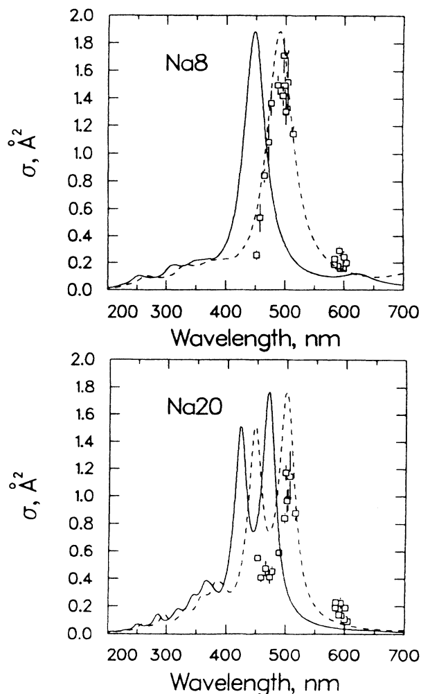
FIG. 3. Photoabsorption cross sections per atom (for \text{Na}_8 and \text{Na}_{20} ) resulting from the folding of the RPA oscillator strengths with Lorentzian shapes normalized to unity are shown (solid line). The widths of the Lorentzians are specified by \Gamma/\hbar\omega_0 \approx 0.1 and 0.06 for \text{Na}_8 and \text{Na}_{20} , respectively (Ref. 5), \hbar\omega_0 being the peak energy of a given Lorentzian. The experimental data (Ref. 16) are also shown. The dashed line is the solid line shifted so that there is a maximum overlap with the data.
