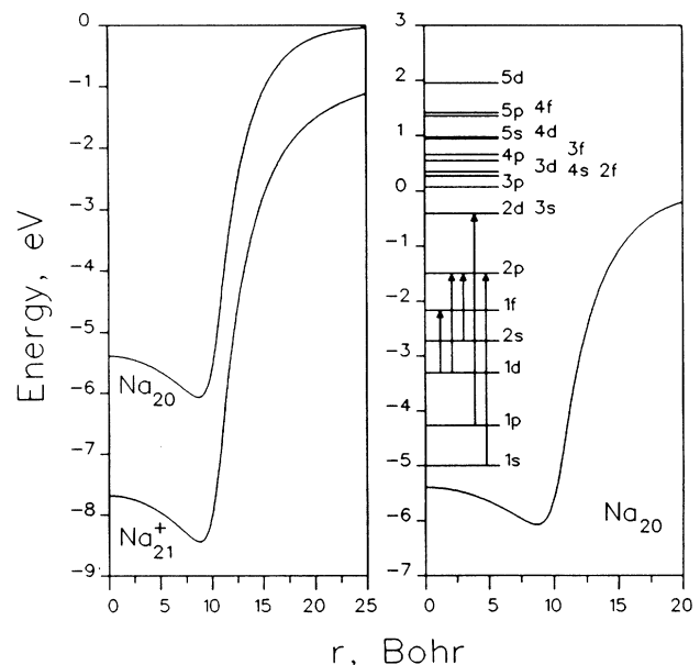
FIG. 1. Self-consistent potentials (Ref. 10) associated with \text{Na}_{20} and \text{Na}_{21}^+ and used in the solution of the single-particle Hamiltonian H_0 appearing in Eq. (1). For \text{Na}_{20} , the resulting single-particle levels relevant to the discussion of the dipole resonance, as well as some of the associated unperturbed particle-hole transitions, are also shown.
