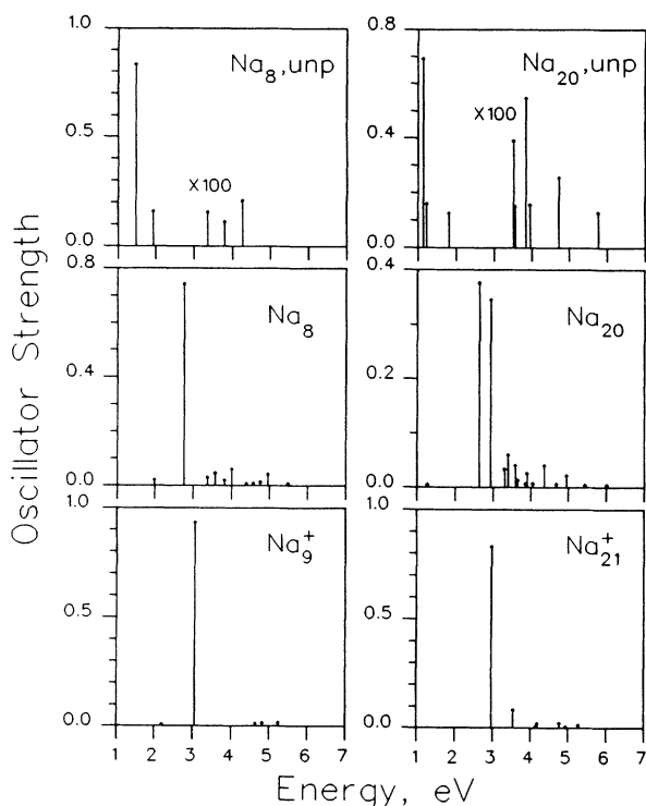
FIG. 2. Oscillator strength function for the photoabsorption of \text{Na}_8 , \text{Na}_{20} , \text{Na}_9^+ , and \text{Na}_{21}^+ clusters. In the upper figures, the unperturbed oscillator strengths for the neutral clusters is displayed. Also, in the upper figures, the strength values above 3 eV have been multiplied by 100.
