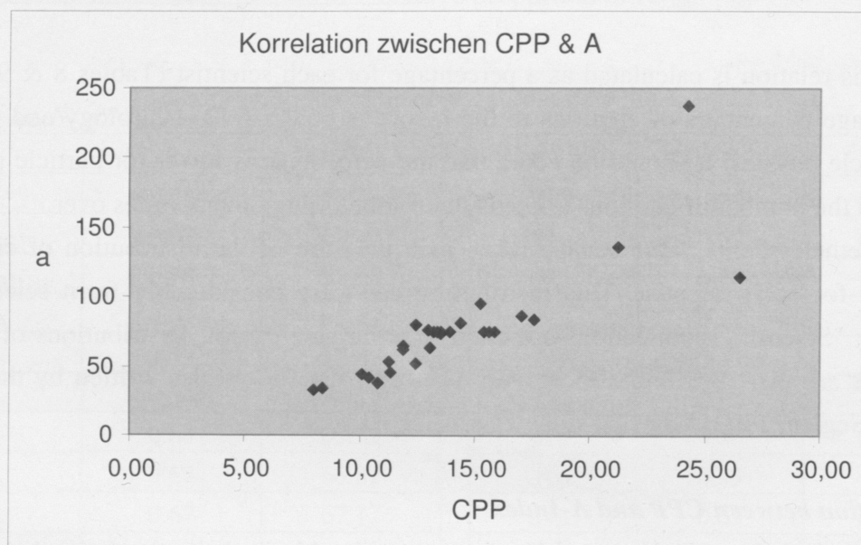
Figure 8. Correlation between CPP and A (particle physics).
