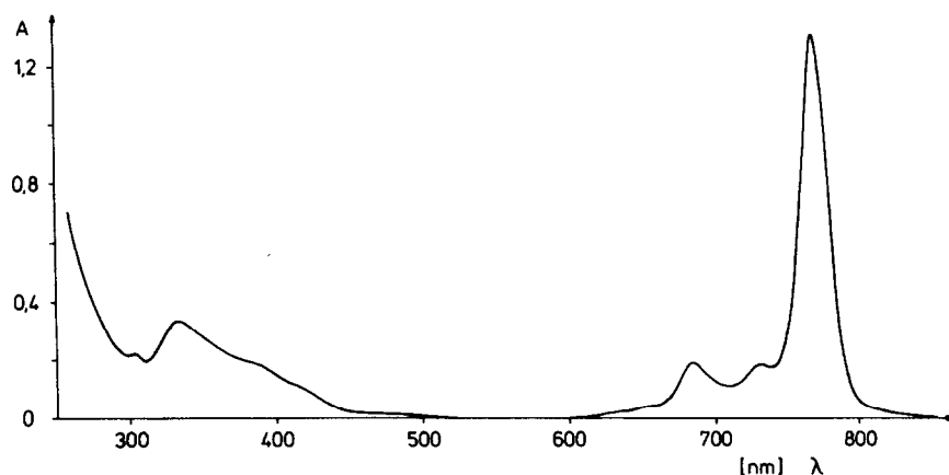
Fig. 1. Absorption spectrum of 8.12 \times 10^{-6} M Zn-2,3-NPC in DMSO; 1 cm cell.
