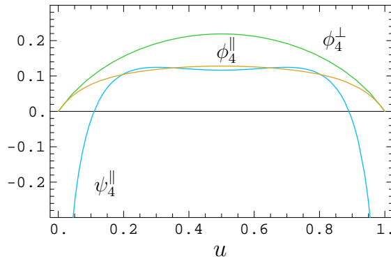
Figure 3: [Colour online] Renormalon-model predictions for \phi_{4;\rho}^{\perp} and \psi_{4;\rho}^{\perp} ; \psi_{4;\rho}^{\perp} = 0 in the renormalon model.
