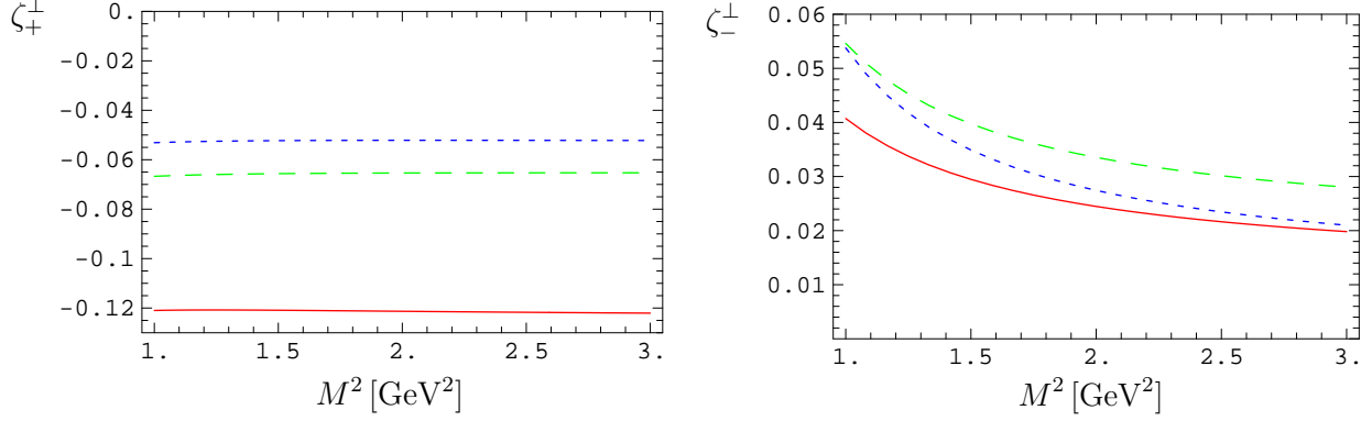
Figure C: [Colour online] \zeta_+^\perp|_{\text{ND,PP}} (left) and \zeta_-^\perp|_{\text{ND,PP}} (right) from the PP sum rule (C.7), as functions of M^2 , for \mu = 1 \text{ GeV} and central values of input parameters. Solid [red] lines: \rho ( s_0 = 1.2 \text{ GeV}^2 ), long dashes [green]: K^* ( s_0 = 1.4 \text{ GeV}^2 ), short dashes [blue]: \phi ( s_0 = 1.8 \text{ GeV}^2 ).
