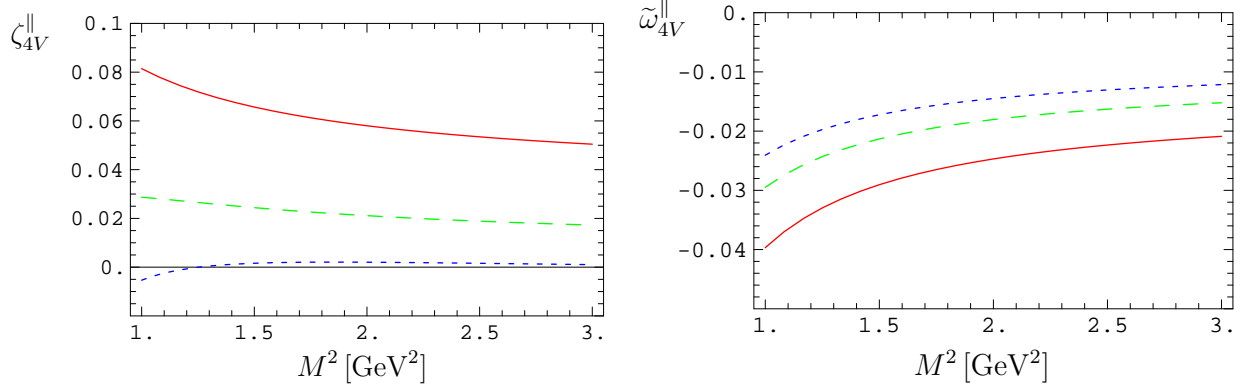
Figure A: [Colour online] \zeta_{4V}^{\parallel} (left) and \tilde{\omega}_{4V}^{\parallel} (right) from the non-diagonal MP sum rules (B.3) and (B.4) as functions of M^2 , for central values of the input parameters. Solid [red] lines: \rho ( s_0 = 1.5 \text{ GeV}^2 ), long dashes [green]: K^* ( s_0 = 1.8 \text{ GeV}^2 ), short dashes [blue]: \phi ( s_0 = 2 \text{ GeV}^2 ). All parameters are evaluated at the scale \mu = 1 \text{ GeV} .
