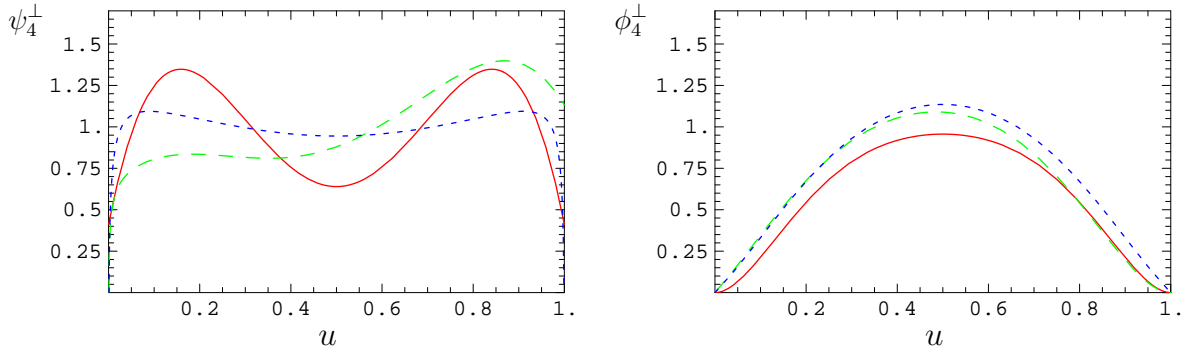
Figure 2: [Colour online] Same as Fig. 1 for \psi_4^{\perp} , (4.24), and \phi_4^{\perp} , (4.25).
