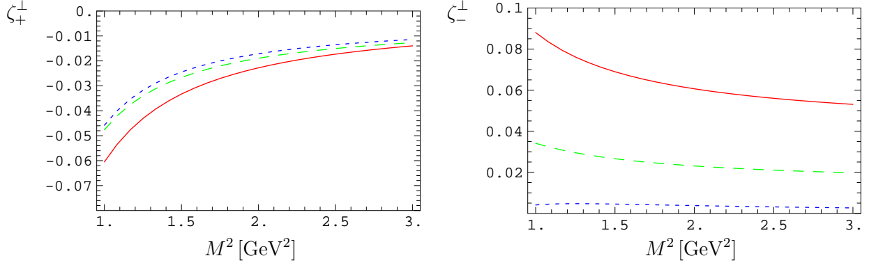
Figure D: [Colour online] \zeta_+^\perp|_{\text{ND,MP}} (left) and \zeta_-^\perp|_{\text{ND,MP}} (right) from the MP sum rule (C.10), as functions of M^2 , for \mu = 1 \text{ GeV} and central values of input parameters. Solid [red] lines: \rho ( s_0 = 1.0 \text{ GeV}^2 ), long dashes [green]: K^* ( s_0 = 1.2 \text{ GeV}^2 ), short dashes [blue]: \phi ( s_0 = 1.5 \text{ GeV}^2 ).
