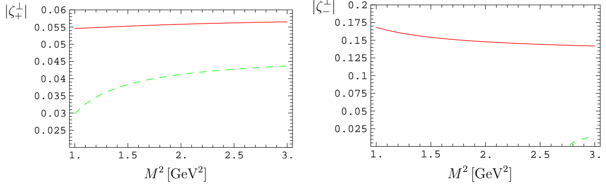
Figure F: [Colour online] |\zeta_+^\perp|_D (left) and |\zeta_-^\perp|_D (right), for the \rho , from the sum rules (C.15) and (C.17). Solid [red] curves: PP ( s_0 = 1.2 \text{ GeV}^2 ), dashed [green] curves: MP sum rules ( s_0 = 1.0 \text{ GeV}^2 ).
