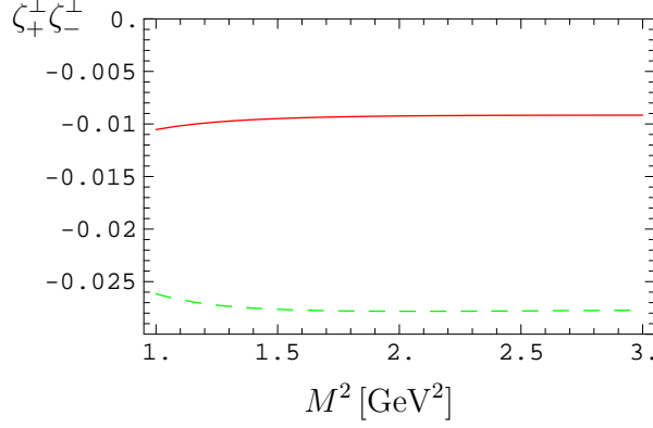
Figure E: [Colour online] (\zeta_+^\perp \zeta_-^\perp)_D for \rho from the PP sum rule (C.16) (solid [red] curve) and the MP sum rule (C.18) (dashed [green] curve).
