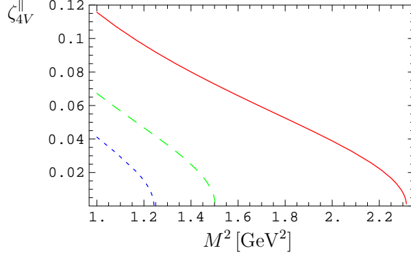
Figure B: [Colour online] \zeta_{4V}^{\parallel} from (B.8). Solid [red] line: \rho , long dashes [green]: K^* , short dashes [blue]: \phi . Same input parameters as in Fig. A.
