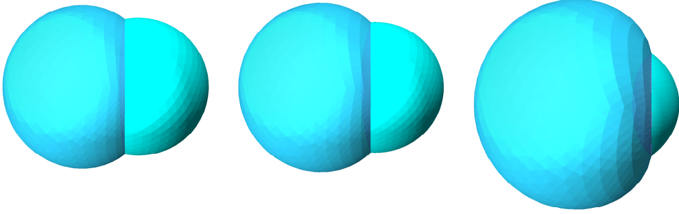
Figure 16: Sintering of two particles for \varsigma = (\frac{5}{4}, \frac{5}{4}, 1) . Solution plotted at times t = 0.1, 0.2, 0.35 .
