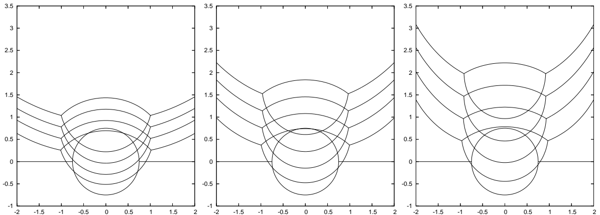
Figure 6: Travelling wave solutions at times t = 0, 1, \dots, 4 for the contact angles \alpha = 60^\circ, 45^\circ, 30^\circ .
