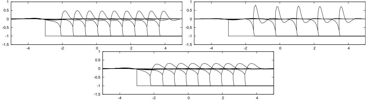
Figure 8: Anisotropic travelling wave solutions at times t = 0, 0.5, \dots, T , with T = 4.5, 2.5, 4.5 , for \varsigma = (1, 1, 1) , \varsigma = (1, 1, 2) and \varsigma = (2, 2, 1) .
