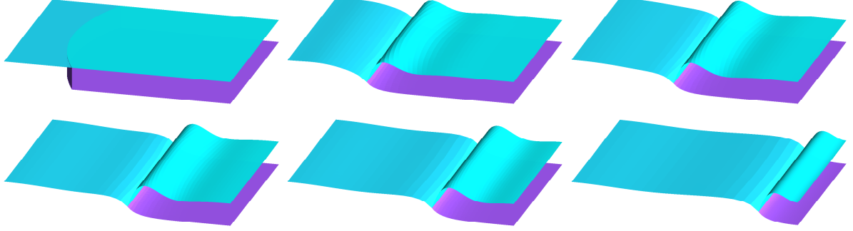
Figure 22: Flattening of the triple junction line profile. Solution plotted at times t = 0, 0.5, 1, 1.5, 2, 3 .
