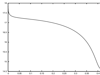
Figure 15: Sintering of two particles. Solution plotted at times t = 0.1, 0.2, 0.35 , with a plot of E(\Gamma^m) below.
