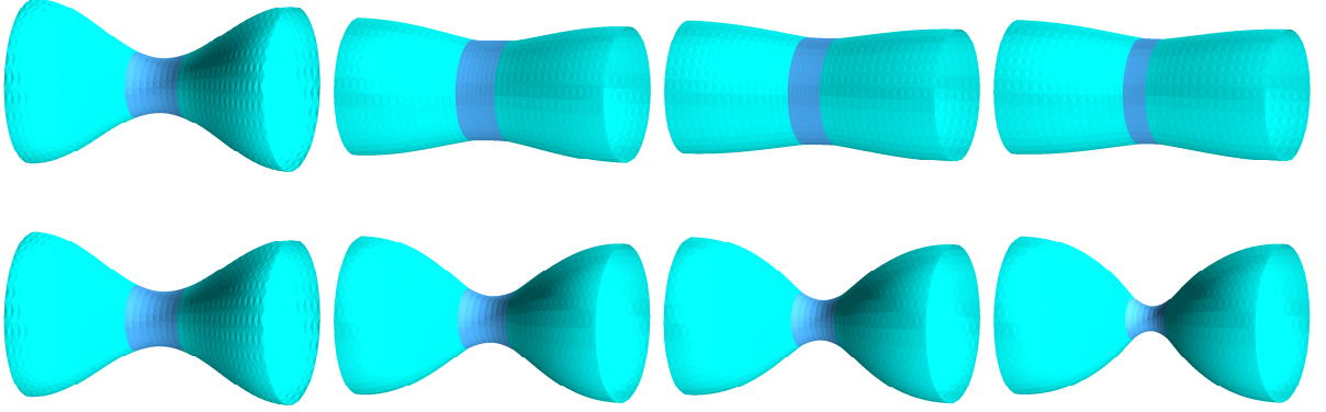
Figure 20: Sintering evolution for \varsigma_s/\varsigma_{gb} = 10 and \beta_s = 10 at times t = 0, 0.05, 0.6, 1.2 . Below the solution at times t = 0, 0.01, 0.03, 0.06 for \beta_s = 1 .
