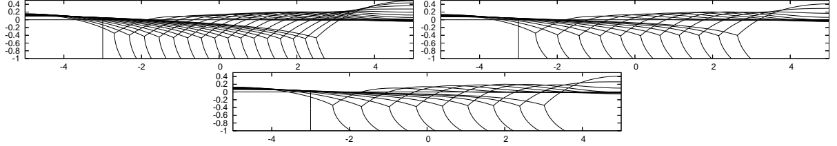
Figure 3: Travelling wave solutions at times t = 0, 0.5, \dots, T , with T = 8, 5.5, 4.4 , for the contact angles \alpha = 60^\circ, 45^\circ, 30^\circ .
