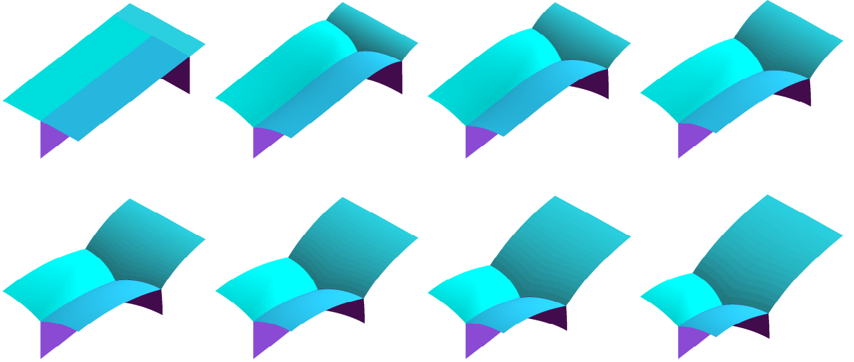
Figure 21: Evolution of three grain boundaries in a tricrystal. Plotted at times t = 0, 0.1, 0.5, 1, 1.5, 2, 2.5, 3 .
