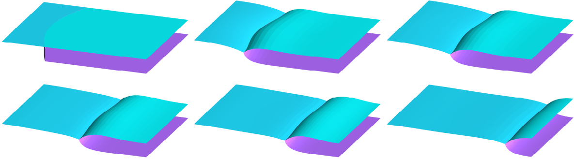
Figure 17: Flattening of the triple junction line profile. Solution plotted at times t = 0, 0.5, 1, 1.5, 2, 3 .
