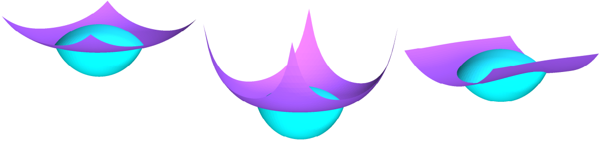
Figure 12: Profile of travelling wave solution at time T = 0.5 . Prescribed contact angles are \alpha = 60^\circ and \alpha = 45^\circ (globally), as well as \alpha = 45^\circ on left/right with \alpha = 90^\circ at front/back.
