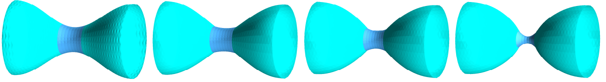
Figure 19: Sintering evolution for \varsigma_s/\varsigma_{gb} = 3 and \beta_s = 1 . Plotted at times t = 0, 0.01, 0.03, 0.05 .
