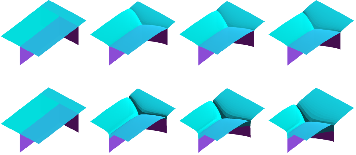
Figure 25: Evolution of three grain boundaries in a tricrystal for anisotropic surface energies. Above \varsigma_s/\varsigma_{gb} = 1/7 = \frac{4}{7} , and below for \varsigma_s/\varsigma_{gb} = 1/2 = \frac{1}{2} . Plotted at times t = 0, 0.1, 0.2, 0.3 .
