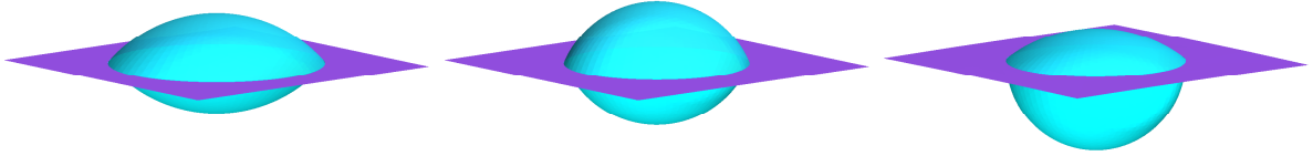
Figure 11: Numerical steady state solutions for \varsigma = (\frac{3}{4}, \frac{3}{4}, 1) and \varsigma = (\frac{5}{4}, \frac{5}{4}, 1) . On the right the solution for \varsigma = (\frac{5}{4}, \frac{3}{4}, 1) .
