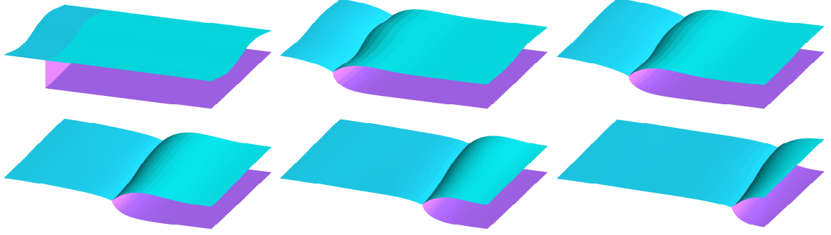
Figure 18: Flattening of the triple junction line profile. Solution plotted at times t = 0, 0.5, 1, 2, 3, 4 .
