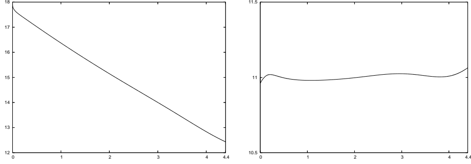
Figure 4: Plots of \tilde{\mathcal{E}}(\Gamma^m) and |\Gamma^m| over time.
