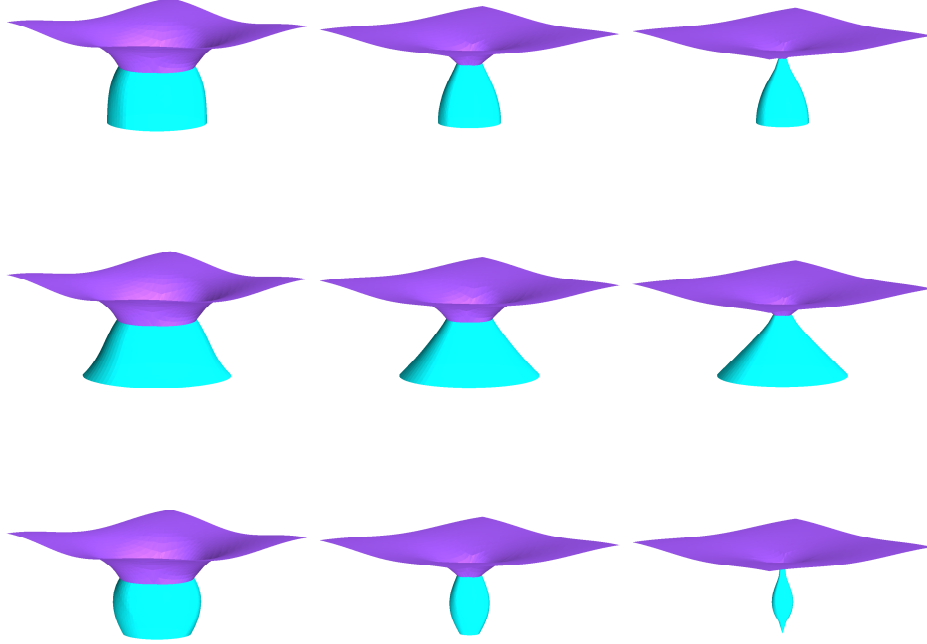
Figure 14: Shrinking of a grain attached to a lower boundary with different contact angles. Solution plotted at times t = 0.05, 0.1, 0.11 ( \alpha = 90^\circ ), t = 0.05, 0.1, 0.13 ( \alpha = 45^\circ ) and t = 0.05, 0.09, 0.1 ( \alpha = 120^\circ ).
