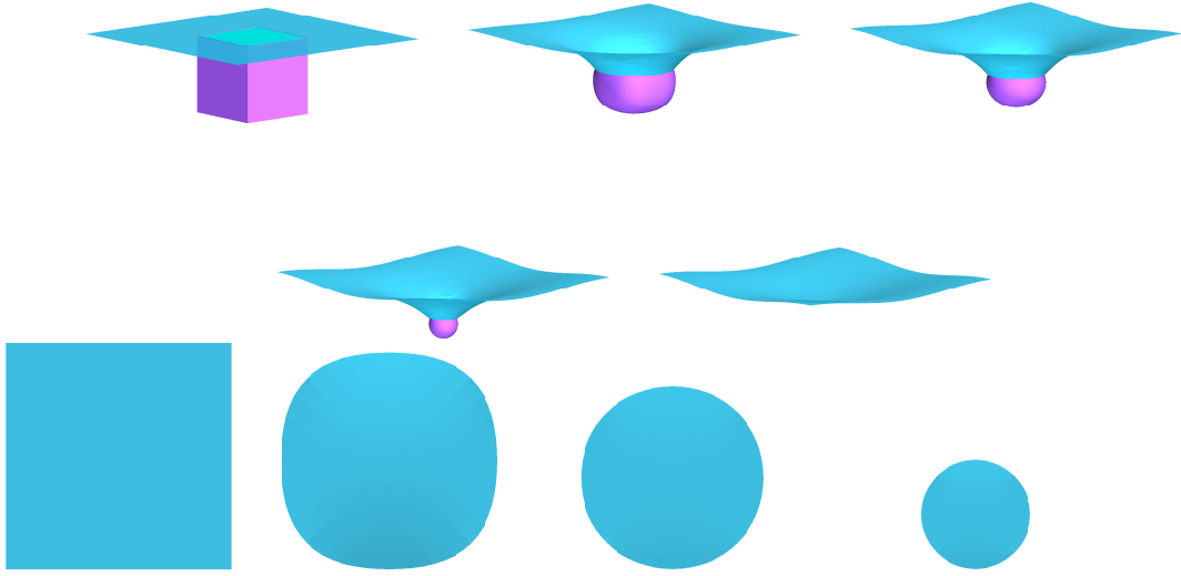
Figure 13: Shrinking of a grain. Solution plotted at times t = 0, 0.025, 0.05, 0.075, 0.1 . Below the surface \Gamma_1^m at these times.
