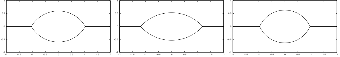
Figure 5: Numerical steady states for \zeta_{gb} = 1 and \zeta_s = 1, \frac{3}{4}, \frac{5}{4} .
