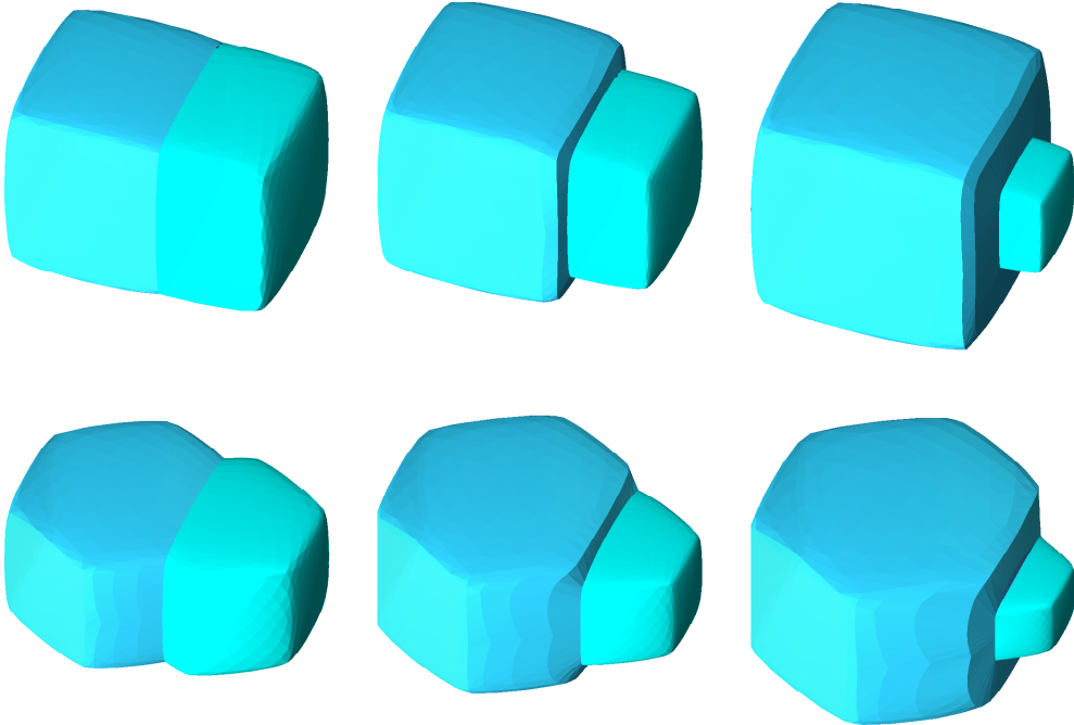
Figure 24: Sintering of two anisotropic particles. Solution plotted at times t = 0.1, 0.7, 0.78 (above) and t = 0.1, 0.3, 0.33 (below).
