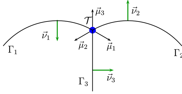
Figure 1: Sketch of the local orientation of (\Gamma_1, \Gamma_2, \Gamma_3) at the triple junction line \mathcal{T} (blue). Depicted above is a plane that is perpendicular to \mathcal{T} .
