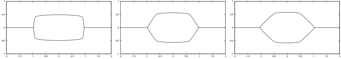
Figure 9: Numerical steady states for different anisotropies.
