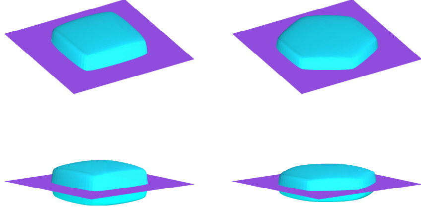
Figure 23: Numerical steady states for different anisotropies. The plots show \Gamma^M from two different points of view.
