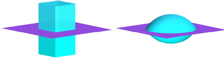
Figure 10: Initial setup and numerically steady state solution for equal surface energies.
