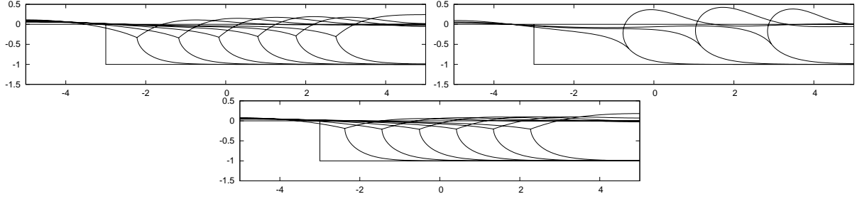
Figure 2: Travelling wave solutions at times t = 0, 0.5, \dots, T , with T = 3, 1.5, 3 , for \varsigma = (1, 1, 1) , \varsigma = (1, 1, 2) and \varsigma = (2, 2, 1) .
