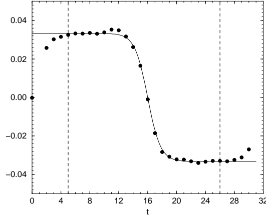
Figure 1: The ratio -\frac{2}{m_V} \frac{1}{3} \sum_i C_{\mathcal{O}_i^a V_i}(t; \vec{0}) / \frac{1}{3} \sum_i C_{V_i V_i}(t; \vec{0}) \equiv \langle \xi \rangle_a^{\parallel} \tanh m_V (\frac{1}{2} N_T - t) versus t for \beta = 5.29 , \kappa_{sea} = 0.1350 , \kappa_{val} = (0.1355, 0.1343) , \vec{p} = \vec{0} . The results are denoted by filled circles. Also shown is a one parameter fit (the m_V mass having been determined previously). The fit range is denoted by vertical dashed lines. The operator has been renormalised to the \overline{MS} scheme at \mu = 2 GeV, so that the value obtained corresponds directly to a point in Fig. 2 (the sixth point from the left).
