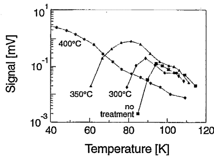
FIG. 2. Photoresponse vs temperature of a 250- \mu\text{m} -wide \text{TiBa}_2\text{Ca}_2\text{Cu}_3\text{O}_9 stripe, for a bias current density of 1 \text{ kA}/\text{cm}^2 , untreated and after subsequent vacuum heat treatments at increasing temperatures.
