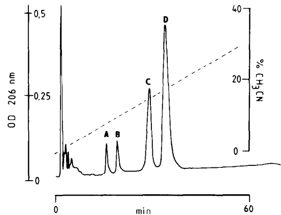
Fig.3. Isolation of tryptic peptides by reversed-phase HPLC derived from deglycosylated I-SG (section 2). Material in peak C and D was submitted to sequence analysis (table 2).
