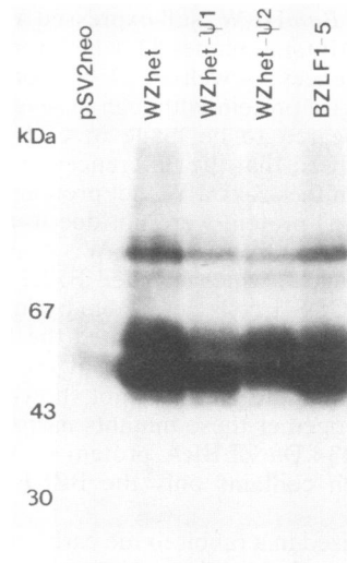
FIG. 7. Induction of replicative antigens by WZhet, two chimeric mutants, and BZLF1; immunoblot of replicative antigens induced in D98/HR-1 cells after transfection with pSV2neo or pSV2neo containing WZhet, the two chimeric mutants (WZhet-psi 1 and WZhet-psi 2), or the BZLF1 open reading frame (BZLF1-5). The polyvalent human antiserum SC was used to detect replicative antigens.
