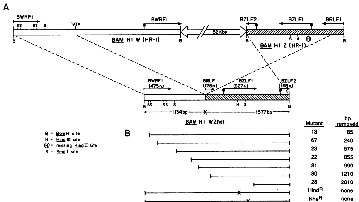
FIG. 1. (A) Diagram of the structure of the Bam HI WZhet fragment, based on its nucleotide sequence (Jenson and Miller, submitted). Letters such as BWRFI and BZLF1 refer to open reading frames in the Cambridge terminology, e.g., BZLF1 is Bam HI-Z leftward frame one (1). Numbers in parentheses (n) are base pairs from each reading frame remaining in WZhet. (B) The location and extent of deletions and site-directed mutations used in this study.
