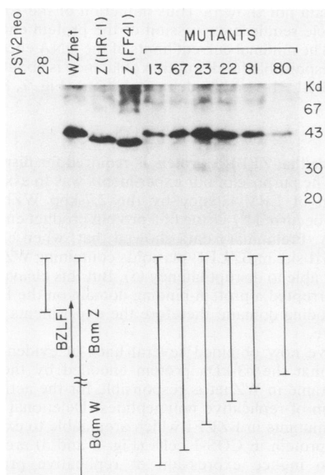
FIG. 3. ZEBRA proteins made in COS-1 cells by WZhet and deletion mutants which invade WZhet from the left end. Note that mutant 80, which eliminates all of the sequences from Bam HI-W, still makes a ZEBRA protein with the electrophoretic mobility of WZhet ZEBRA protein. Mutant 28, which invades BZLF1, makes no protein.
