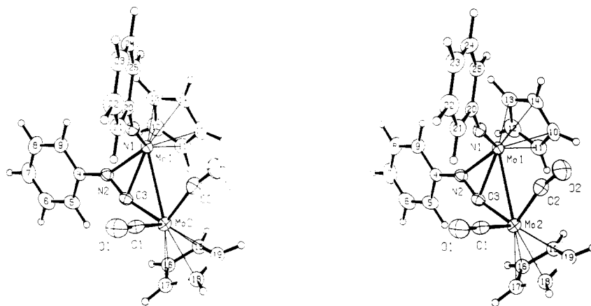
Figure 1. Stereoscopic view of the molecule of II.
