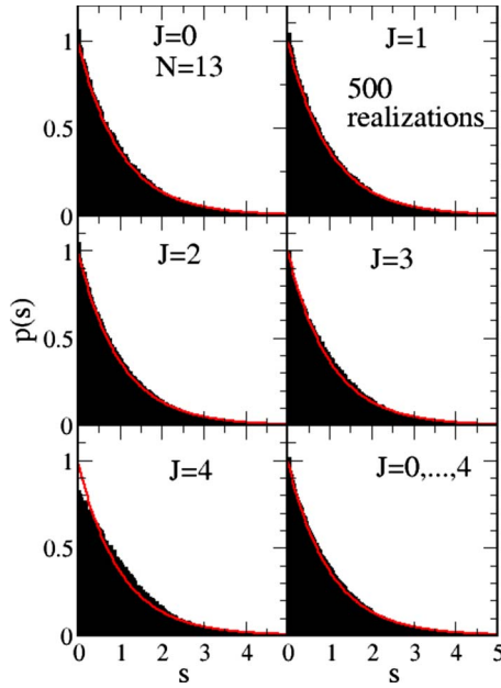
FIG. 1. (Color online) Nearest-neighbor level spacing for a system of a single central spin S_1=1/2 and 13 bath spins of length l=1/2 . The red curve is the exponential p(s)=e^{-s} .
