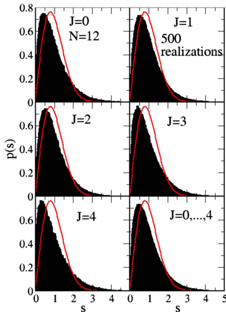
FIG. 2. (Color online) Nearest-neighbor level spacing for a system of two central spins S_1=S_2=1/2 and 12 bath spins of length l=1/2 . The red curve is the GOE Wigner surmise.
