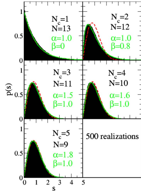
FIG. 4. (Color online) Joint level spacing distribution for J=0, \dots, 4 and increasing number of central spins. The red dashed lines are the exponential function ( N_c=1 ) and the Wigner surmise ( N_c>1 ). The green solid lines are a fit to generalized Brody distribution (2).
