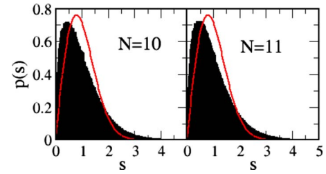
FIG. 3. (Color online) The same data as in the bottom right panel of Fig. 2 but for N=10 and N=11 bath spins.
