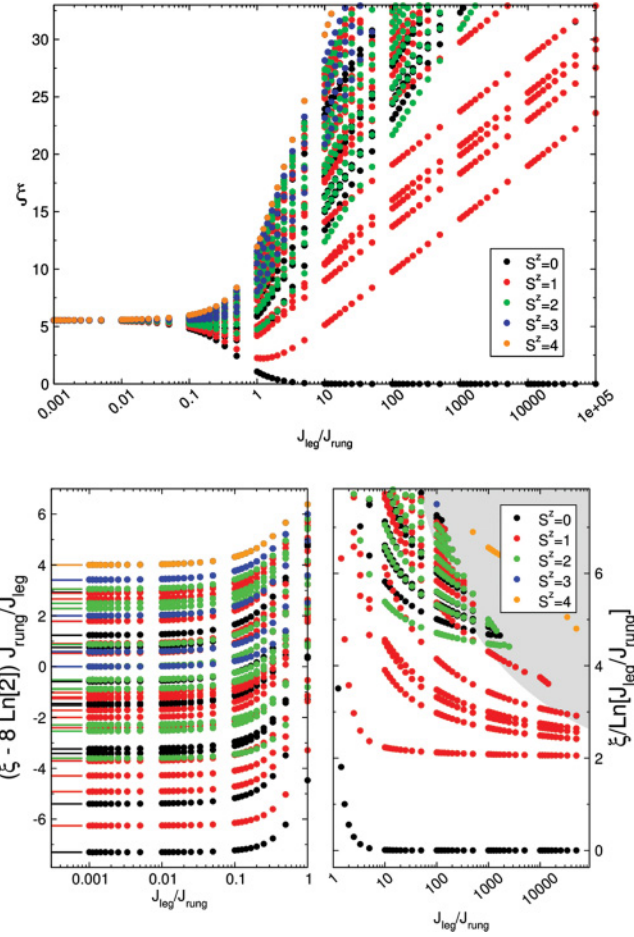
FIG. 2. (Color online) Overview of the entanglement spectrum of the reduced density matrix of a single chain (cf. setup in Fig. 1) in a Heisenberg ( \Delta = 1 ) spin ladder for different S_{\text{tot}}^z = S_{\text{tot}} sectors as a function of J_{\text{leg}}/J_{\text{rung}} . The system size is L = 8 . While in the upper panel the bare entanglement spectrum is shown, in the lower panels the leading asymptotic behavior in the two limiting cases J_{\text{leg}}/J_{\text{rung}} \rightarrow 0 and J_{\text{rung}}/J_{\text{leg}} \rightarrow 0 is highlighted by appropriate shifts and rescaling indicated on the y axes. The filled dots in all panels denote numerical entanglement spectrum levels, while the constant lines in the lower left panel highlight twice the eigenvalues of a single L = 8 , S = 1/2 Heisenberg chain. The gray region in the lower right panel indicates the part of the rescaled entanglement spectrum affected by the finite (double) precision arithmetic used in the numerical calculations.
