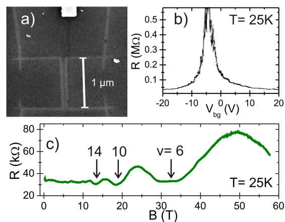
FIG. 1: (color online). (a) Scanning electron microscope image of a typical sample. The length of the GNRs is 1 \mu\text{m} , the width 70 nm. In the upper part of the image a palladium contact is visible. (b) Two-terminal resistance as a function of V_{bg} at T = 25 K and zero magnetic field. (c) Magnetoresistance trace at V_{bg} = -20 V, showing quantum Hall features at \nu = 6, 10 and 14 .
