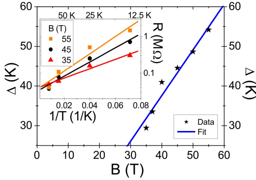
FIG. 4: (color online). Energy gaps \Delta extracted from the slope of the Arrhenius plot for T \geq 14 K (inset). The full line represents a linear fit to the data.
