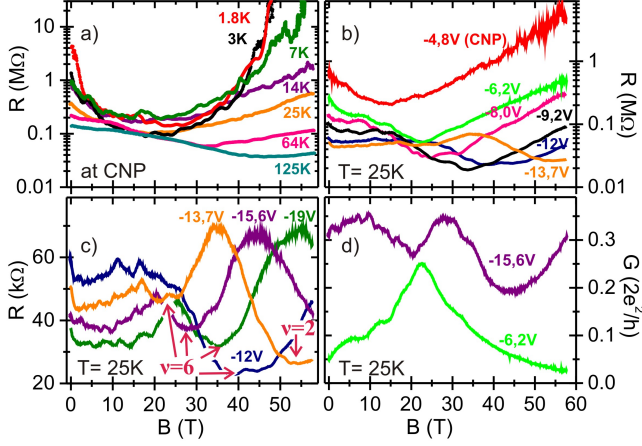
FIG. 2: (color). (a) Magnetoresistance of the GNR for various temperatures at the charge neutrality point. (b) Magnetoresistance for different gate voltages close to the CNP and (c) further away from the CNP at T = 25 K. The arrows and the numbers indicate the corresponding filling factors \nu of the quantum Hall state, \nu = 2 and 6 . (d) Conductance as a function of magnetic field for V_{bg} = -15.6 and -6.2 V.
