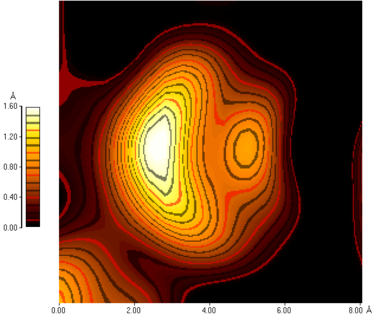
Fig. 11 Topographic image of a single adatom on Si(111)-(7×7) observed by FM-AFM, presumably imaged with a (001) oriented Si tip. The following imaging parameters were used: k = 1800 N/m, A = 8 Å, f_0 = 16860 Hz, \Delta f = -160 Hz, rms frequency error \delta \Delta f = 9 Hz, scanning speed = 80 nm/s, sample voltage U = 1.6 V, scanning direction: left to right.
