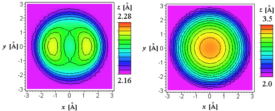
Fig. 12. Simulation of a topographic FM-AFM image of a single adatom on Si(111)-(7×7). Parameters (Left): \gamma = -387 \text{ fNm}^{1/2} , A = 8 Å, short-range force: Stillinger Weber, tip geometry shown in Fig. 17, long-range force = -3.66 \times 10^{-26} \text{ Jm}/(z + \Delta)^2 , \Delta = 5 Å. Parameters (Right): \gamma = -4 \text{ fNm}^{1/2} , A = 8 Å, short-range force: Stillinger Weber, tip geometry shown in Fig. 17, long-range force = -3.66 \times 10^{-28} \text{ Jm}/(z + \Delta)^2 , \Delta = 5 Å.
