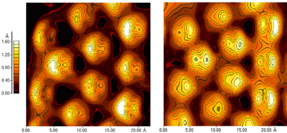
Fig. 9 Topographic image of Si(111)-(7 \times 7) observed by FM-AFM, presumably imaged with a (001) oriented Si tip. Imaging parameters: k = 1800 \text{ N/m} , A = 8 \text{ \AA} , f_0 = 16860 \text{ Hz} , \Delta f = -160 \text{ Hz} , rms frequency error \delta \Delta f = 9 \text{ Hz} , scanning speed = 80 nm/s, sample voltage U = 1.6 \text{ V} .
