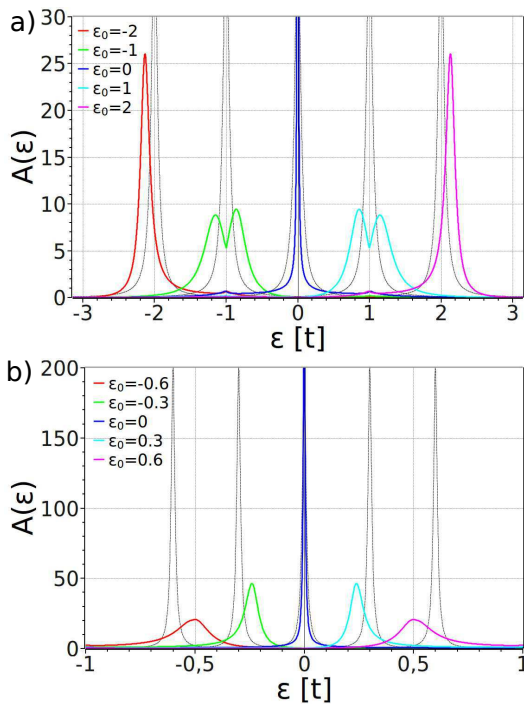
Figure 4: (Color online) Spectral function of a single level coupled to armchair edges. The equidistant dashed lines show the position of the level in the wide-band limit. V_0 = 0.1t
