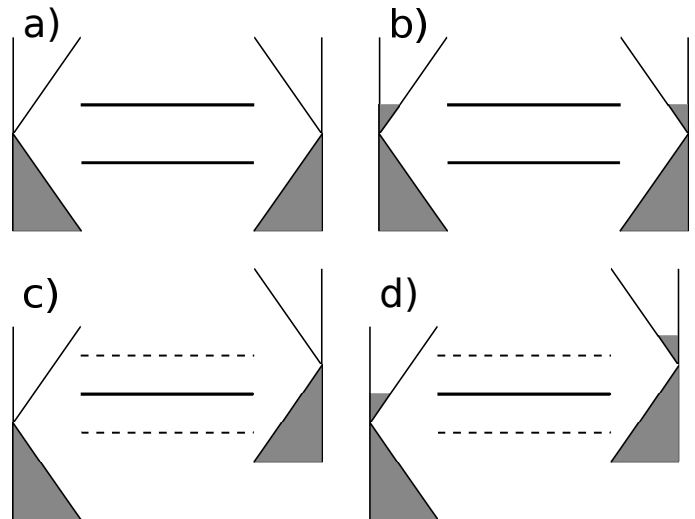
Figure 8: The energy level diagrams corresponding to the points a)-d) marked in Fig. 7c of the differential conductance for zigzag electrodes.
