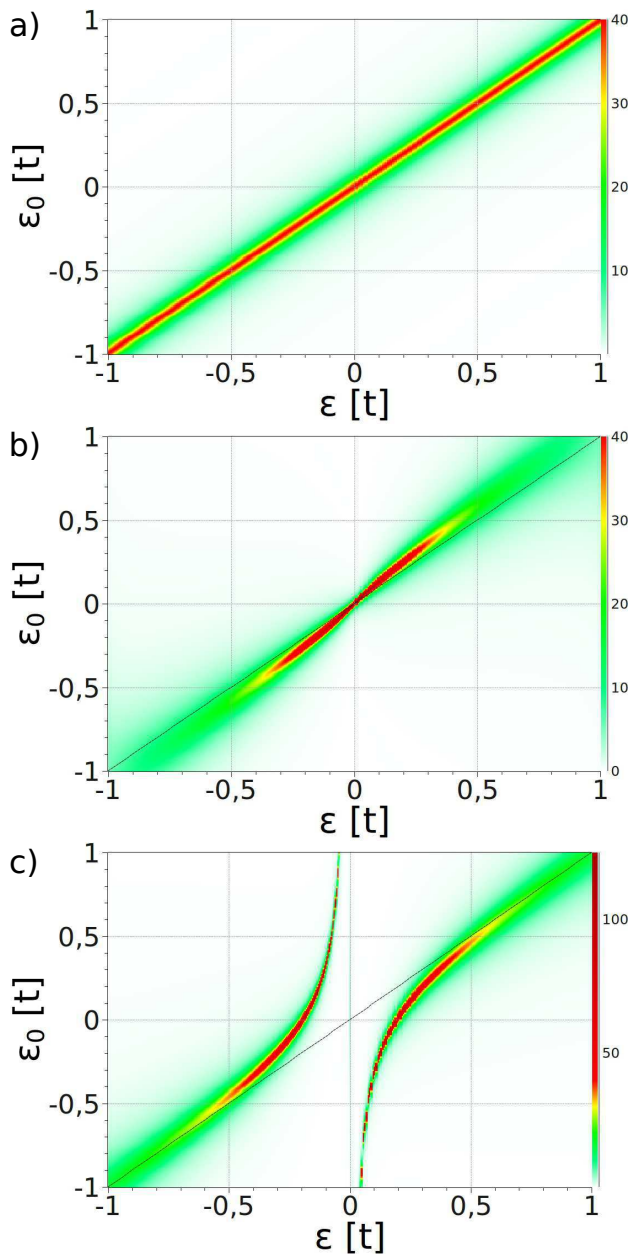
Figure 6: (Color online) Color-coded strength of spectral function of a single level coupled to wide-band leads (a), armchair leads (b) and zigzag leads (c).
