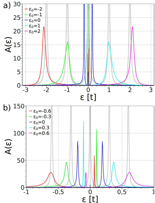
Figure 5: (Color online) Spectral function of a single level coupled to zigzag edges. The dashed lines show the position of the levels in the wide-band limit. V_0 = 0.1t
