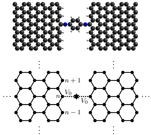
Figure 1: (Color online) Example of a plane graphene molecular junction and schematic representation (lower panel) of the considered single-level model (for zigzag edge).
