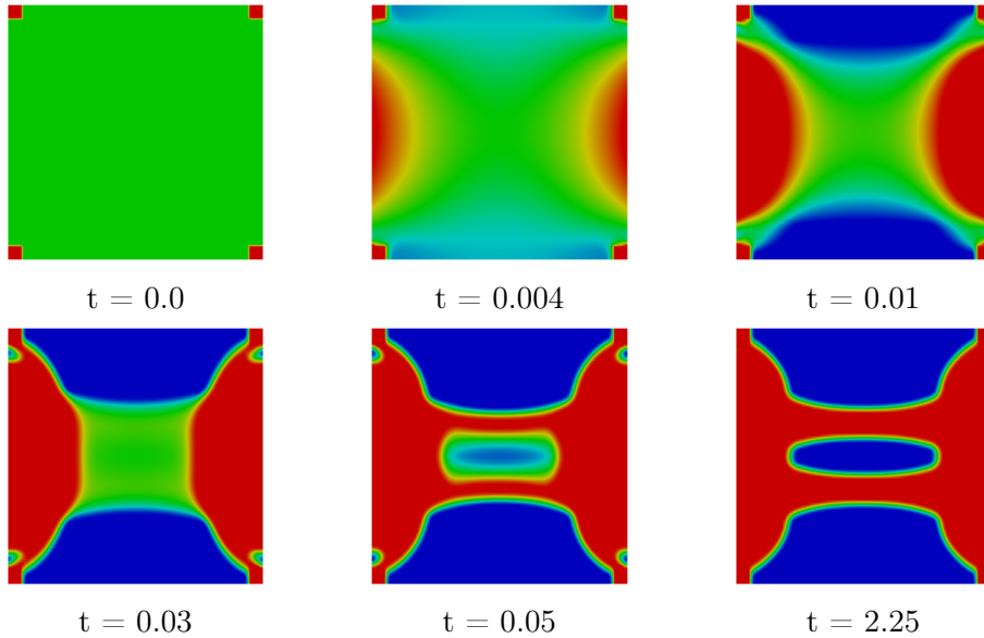
Figure 9: Push simulation with N = 2 and \varphi_h^0 = (\frac{1}{2}, \frac{1}{2})^T on \Omega \setminus S_0 , material in red and void in blue.
