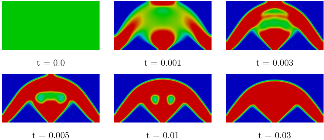
Figure 2: Bridge simulation with N = 2 and \varphi_h^0 \equiv (\frac{1}{2}, \frac{1}{2})^T , material in red and void in blue.
