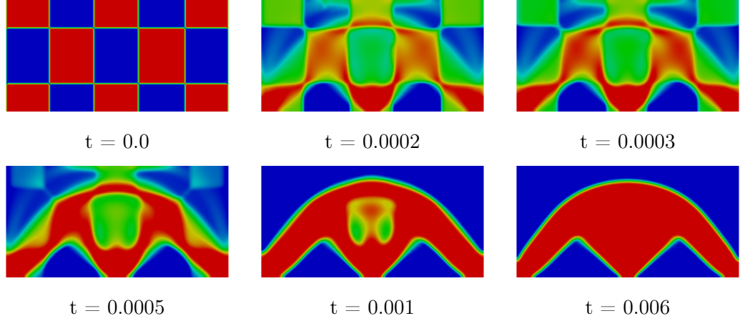
Figure 3: Bridge simulation with N = 2 and checkerboard initial data, material in red and void in blue.
