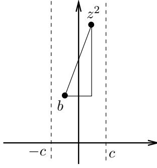
FIGURE 3. Estimating the argument of z^2 - b .
