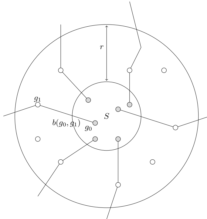
Figure 6.2: Whyte's vanishing criterion
