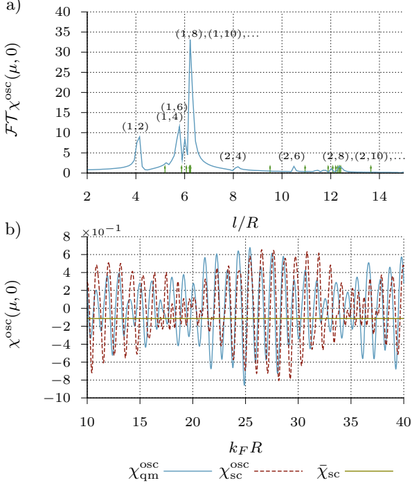
FIG. 13: a) Length spectrum of \chi^{\text{osc}} calculated quantum mechanically from the eigenenergies of a graphene disk, Eq. (78), at \phi = 0 , 1/\beta \approx 10^{-3} t and using R \approx 200 a . Peak positions correspond to orbit families (w, v) . Due to pseudospin interference, orbits with an odd number of reflections do not contribute. Their lengths are marked by green arrows. b) Comparison of the semiclassical prediction (84) (red dashed line) for the orbital magnetic susceptibility with the quantum mechanical result (solid blue) at B = 0 and 1/\beta \approx 10^{-3} t . The (green) horizontal line represents the typical value, Eq. (88), of the magnetic susceptibility. All susceptibilities are normalized by X = \chi_0(\phi_0/(2\mathcal{A})) and \sqrt{k_F R} .
