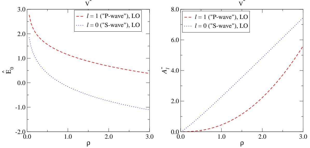
Figure 3: Left: The lowest “ S -wave” and “ P -wave” eigenvalues obtained with the LO potential V_{\text{LO}}^- (cf. eq. (6.31)). Right: The “amplitudes” corresponding to the lowest eigenmodes (cf. eq. (7.15)).
