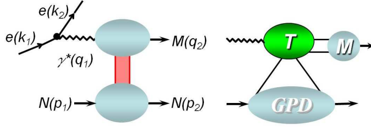
Figure 1: DVMP process from the t -channel view (left) and partonic view (right).
