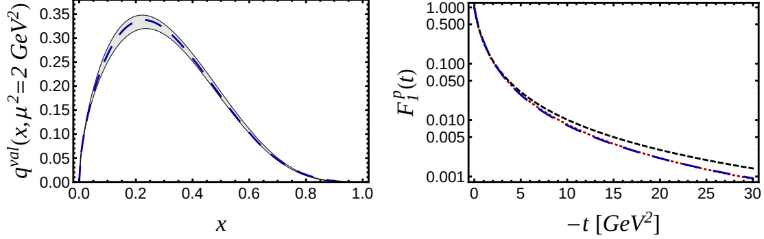
Figure 3: A simple GPD model (long dashed), based on the ansatz (5.5), versus Alekhins LO PDF parameterization [122] (grayed area) [left panel] and Kelly's [123] (dotted) [Sachs (short dashed)] form factor parameterization [right panel].
