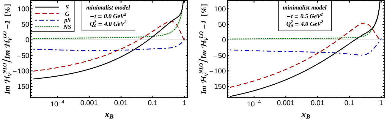
Figure 6: Relative NLO corrections to the imaginary part of the flavor singlet TFF \mathcal{F}_V^S (solid) broken down to the gluon (dashed), pure singlet quark (dash-dotted) and ‘non-singlet’ quark (dotted) at t = 0 \text{ GeV}^2 (left panel) and t = -0.5 \text{ GeV}^2 (right panel) at the initial scale Q_0^2 = 4 \text{ GeV}^2 .
