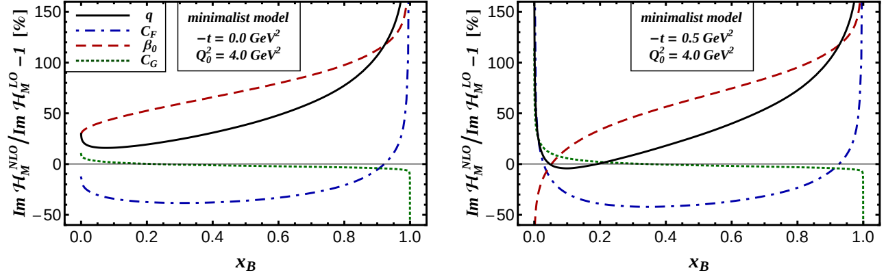
Figure 4: Relative NLO corrections to the imaginary part of the TFF \mathcal{H}_M^{u(-)} (solid) broken down to the C_F (dash-dotted), \beta_0 (dashed), and C_G (dotted) parts at t = 0 \text{ GeV}^2 (left panel) and t = -0.5 \text{ GeV}^2 (right panel) at the initial scale Q_0^2 = 4 \text{ GeV}^2 with four active quarks.
