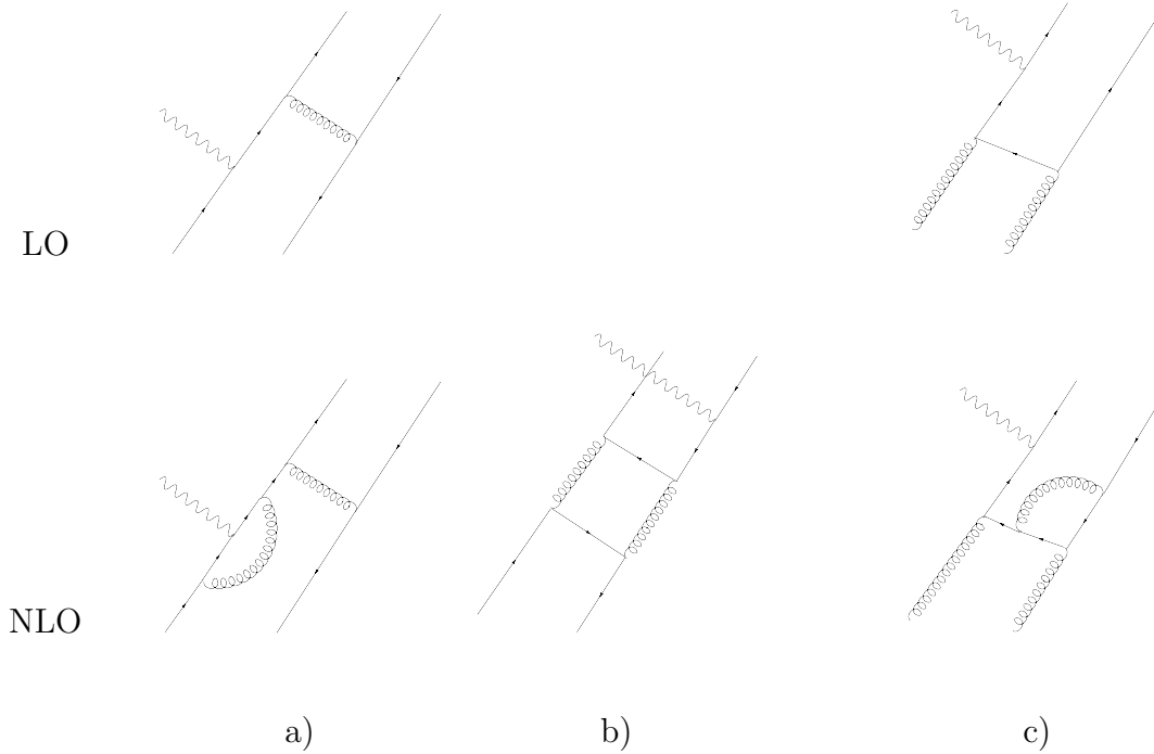
Figure 2: Representative partonic subdiagrams that contribute to DVMP of neutral vector mesons. In context of the GPD part, i.e., partons coming from the proton, (lower "legs", while the upper ones denote the meson) the contributions are organized as: a) quark contribution b) pure singlet quark contribution c) gluon contribution.
