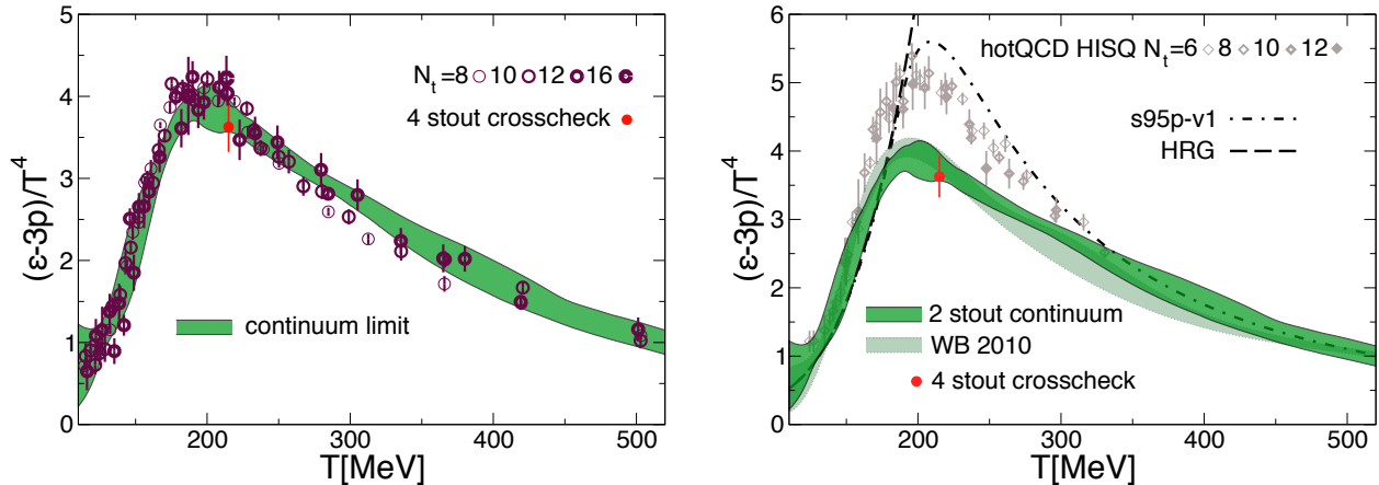
Figure 3: Left: the trace anomaly as a function of the temperature for N_t = 8, 10, 12 and 16 lattices. The continuum extrapolated result including all systematic uncertainties is shown by the shaded band. Using a different action (see text), we performed a continuum extrapolation at the fixed temperature value of 214 MeV, indicated here with a smaller filled red point. This independent result serves as a crosscheck on the peak’s height (also on r.h.s.). Right: comparison of the result with the parallel effort using the HISQ action by the hotQCD collaboration (as it was presented at the Lattice 2012 conference [28], with f_K scale setting) and the related parametrization ‘s95p-v1’ of [29]. A comparison to the Hadron Resonance Gas model’s prediction and our result [14] from 2010 (“WB 2010”) is also shown.
