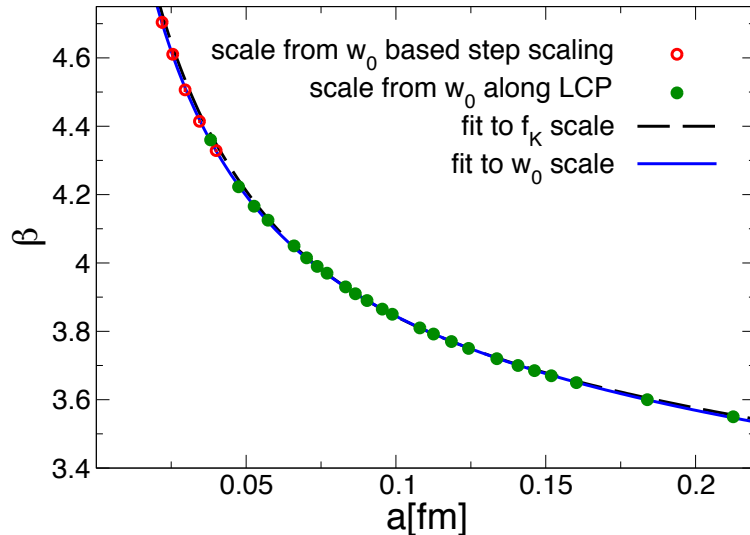
Figure 1: The lattice spacing a for the \beta range used in this paper. Down to a = 0.047 fm two quantities were used to determine the scale, f_K and w_0 . For higher couplings a step-scaling approach was applied.
