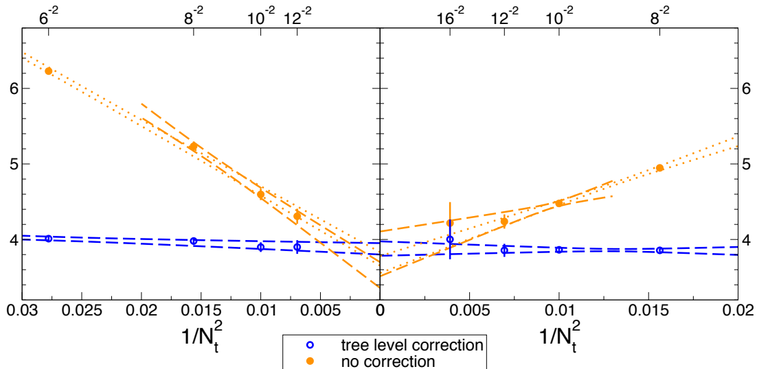
Figure 4: Continuum extrapolation of the trace anomaly at T \approx 214 MeV with (blue points) and without (orange points) tree level improvement. The left panel shows our results with 2+1+1 flavors of 4-step stout improved staggered quarks extrapolating from N_t = 6, 8, 10 and 12 , whereas on the right panel N_f = 2+1 2-step stout improved quarks are used on N_t = 8, 10, 12 and 16 .
