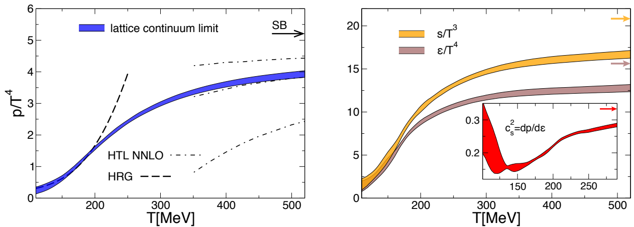
Figure 6: Left: continuum extrapolated result for the pressure with N_f = 2 + 1 flavors. The HRG prediction is indicated by the black line at low temperatures, at high temperature we show a comparison to the NNLO Hard Thermal Loop result of ref. [31] using three different renormalization scales ( \mu = \pi T, 2\pi T or 4\pi T ). Right: entropy and energy density. The insert shows the speed of sound.
