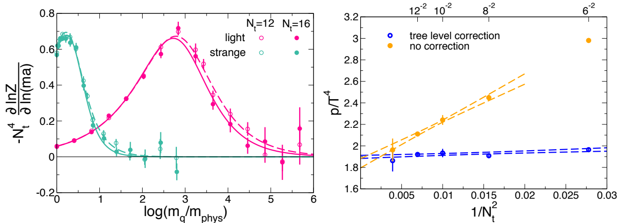
Figure 5: Left: contributions of the light (magenta) and strange quarks (turquoise) to the the pressure at T = 214 MeV at our two finest lattice spacings. The curves represent a scan though various theories with different masses. The sum of the area under the curves gives p/T^4 . Right: continuum extrapolation of the pressure at T \approx 214 MeV with (blue) and without (orange) tree level improvement. Only statistical errors are shown.
