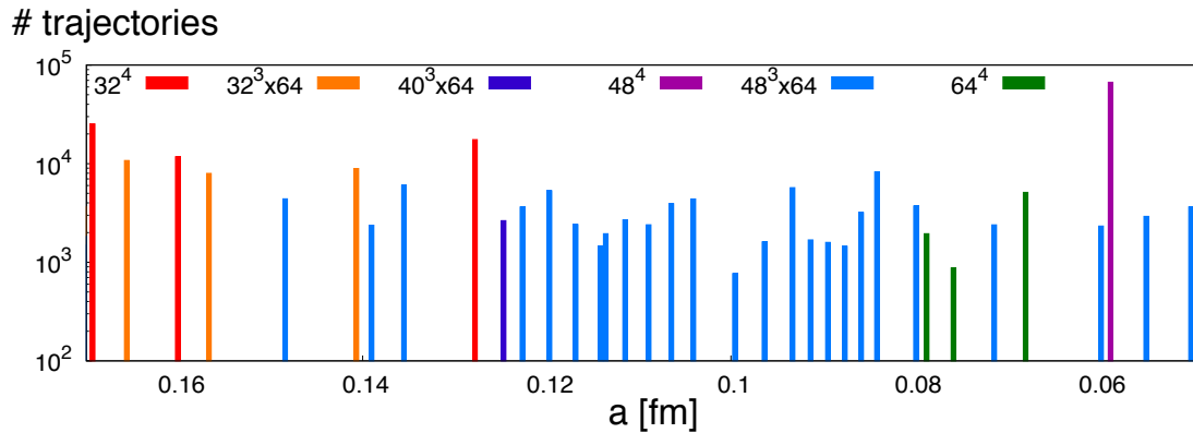
Figure 2: The T = 0 lattices and the collected statistics at various lattice spacings.
