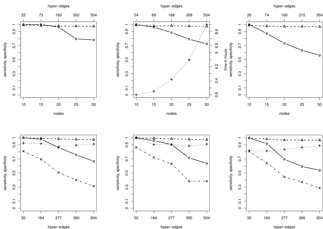
Fig. 3. Simulation results From left to right we set \sigma = 0.5, 1, 2 in each column respectively. Top : Random GTN of n nodes (x-axis) and the median sensitivity, specificity of the ERS (solid circle, dashed triangle) and running time (dotted cross) for ten runs. The top axis shows the mean PKN size. Bottom : Results for ten runs each given a fixed GTN and different PKN sizes (x-axis) including the GTN. Median sensitivity and specificity of the ERS (solid circle, dashed triangle) and the hyper-edges (dotted cross, dashed-dotted x).
