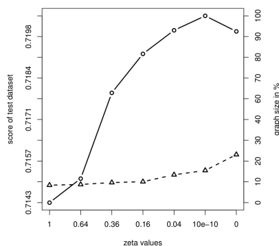
Fig. 5. \zeta calibration Mean cross validated network scores as a function of the complexity parameter \zeta . Score on the test dataset (solid circle, log-scale) and graph size in percent (dashed triangle).
