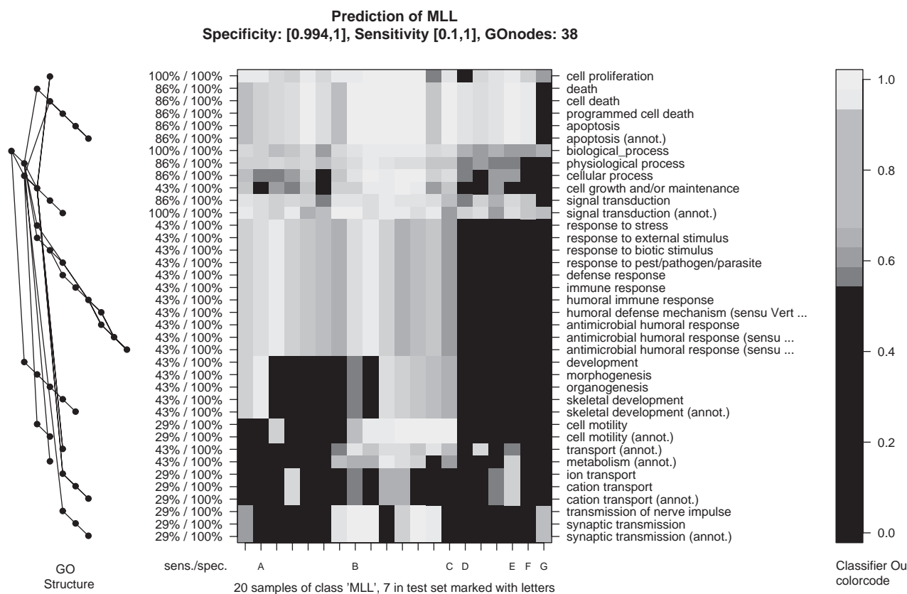
Fig. 2. Structured analysis of 327 acute lymphocytic leukemia patients. Molecular symptoms specific for MLL are shown. They are filtered by minimum specificity.
