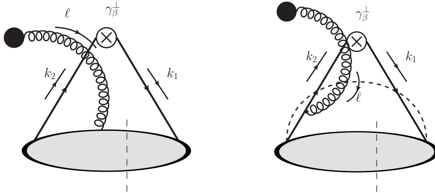
FIG. 1: The Feynman diagrams which contribute to the polarized Drell-Yan hadron tensor.
