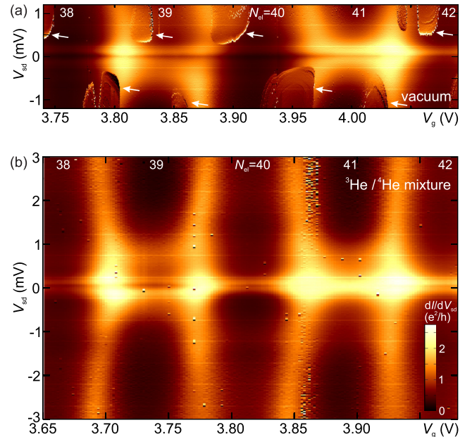
FIG. 3. (a) Numerically derived differential conductance dI/dV_{sd} as function of bias voltage V_{sd} and gate voltage V_g . The device is in vacuum. Kondo ridges of enhanced conductance 18,20,22 are clearly visible; the dark line of lower conductance at V_{sd} = 0 reflects the superconducting energy gap of the rhenium contacts. At finite bias, distinct switching phenomena due to electromechanical feedback 8,13,17 are clearly visible (white arrows). Related data have already been published in Figure 2 of Ref. 13. (b) Comparable measurement of the same sample, but now immersed into the liquid ^3\text{He}/^4\text{He} mixture of a dilution refrigerator; same V_{sd} scaling. The switching phenomena are clearly absent even for significantly higher bias voltage V_{sd} .
