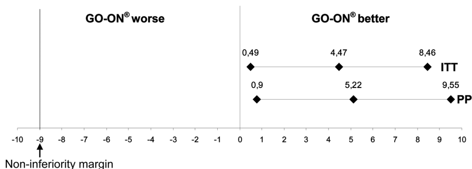
Figure 3 Point estimate and 95% CI of the difference (GO-ON vs Hyalgan, in mm) in the primary outcome represented by the Western Ontario and McMaster Universities pain subscale mean improvement. Values are differences in mean changes between GO-ON and Hyalgan at 6 months after treatment in the per-protocol (PP) and intention-to-treat (ITT) populations ( -9 mm was the non-inferiority margin).
