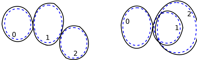
FIG. 4: Long periodic orbit (solid curve) composed of three shorter periodic orbits “0”, “1” and “2” (dashed) by means of two separate (left) or overlapping (right) 2-encounters.
