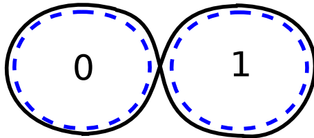
FIG. 3: Sketch of a periodic orbit possessing one 2-encounter as considered for resummation in Sec. III.
