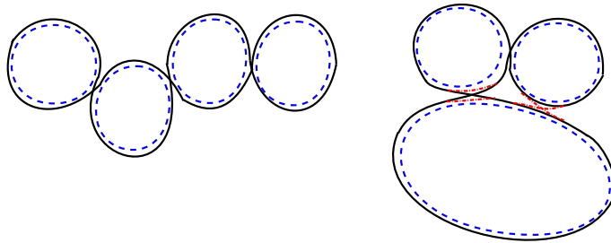
FIG. 5: Left panel: One long, fully connected periodic orbit (full line) surrounds all shorter periodic orbits (dashed lines). Right panel: Two different configurations of connected orbits can be constructed surrounding the shorter periodic orbits. (indicated by the full and dashed dotted lines).
