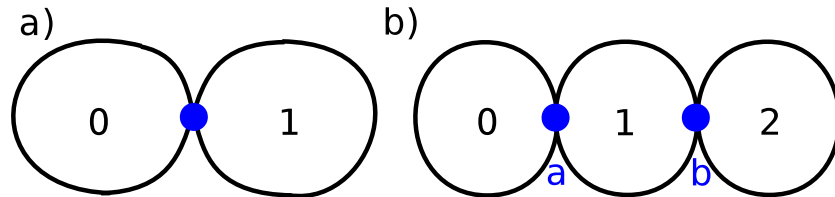
FIG. 2: Two simple quantum graph structures: In a) a directed graph connects 2 bonds “0” and “1” at one vertex. In b) the directed quantum graph consists of two vertices a and b connected by 4 bonds.
