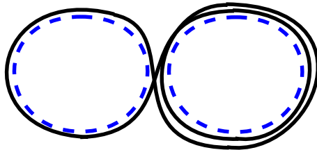
FIG. 1: Partial repetitions of a periodic orbit: A longer orbit (solid curve) comprising a 2-encounter formed by two shorter periodic orbits (dashed lines) traverses one of the shorter periodic orbits twice (dashed).
