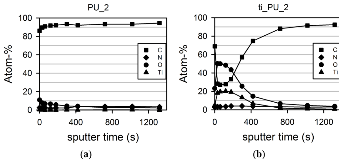
Figure 1. Representative XPS of (a) pure and (b) titaniferous upgraded PU_2. Surface characteristics show a homogenous composition of carbon (C), oxygen (O), titanium (Ti) and nitrogen (N) on titaniferous upgraded ti_PU_2 and pure PU_2 (control). The spectrum of the upgraded surface which can be regarded lies in the measuring range between 30 and 1000 sputtering seconds.
