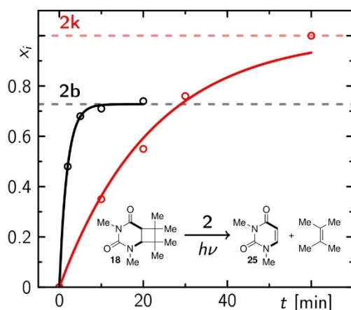
Figure 5. Course of photocycloelimination of 18 mediated by 2b and 2k .
