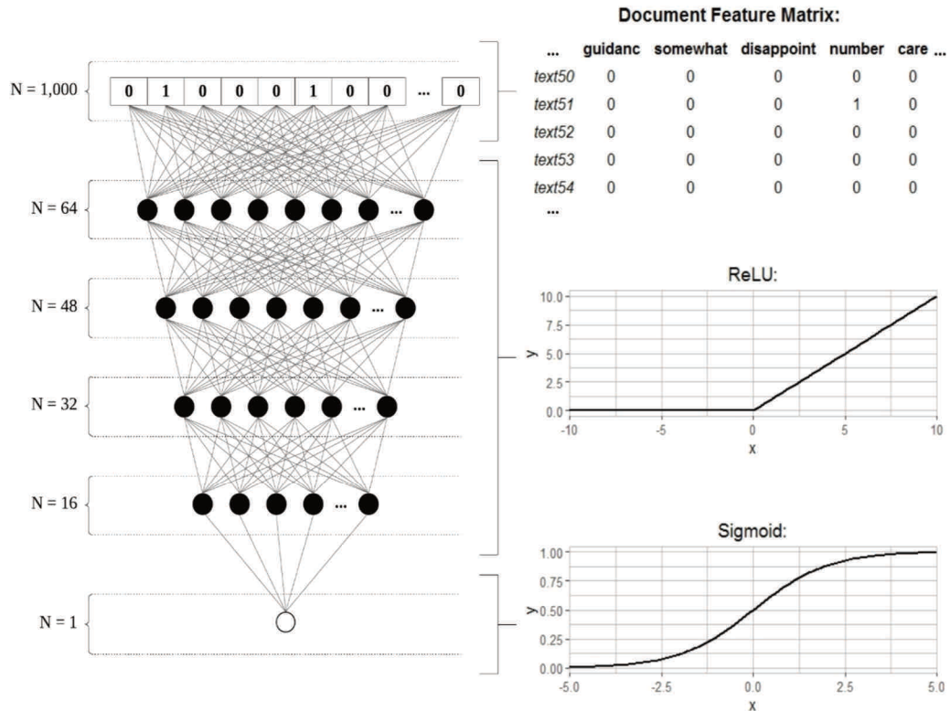
Figure 3.1: ANN Layout
