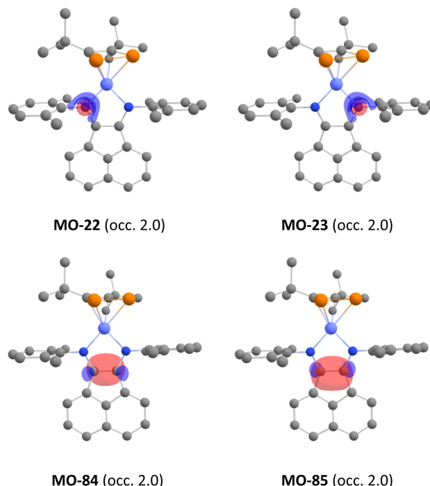
Figure 9. Selected localised molecular orbitals below the active space of a CASSCF calculation [RJCOSX/TZVP-def2/JK, CP(PPP) on Co] on [(\text{DmpBIAN})\text{Co}(1,2\text{-tBu}_2\text{C}_2\text{P}_2)]^- . The occupancy of each orbital is given in parentheses (2.0). Isosurface value for MO-22 and MO-23: 0.0075; for MO-84 and MO-85: 0.06.
