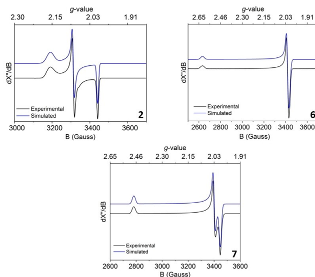
Figure 7. Experimental and simulated X-band EPR spectrum of 2 (top left), 6 (top right) and 7 (bottom) in a 2-methyl-THF glass. 2 : temperature: 10 K, Freq.: 9.646813 GHz, power: 0.2000 mW, mod. amp: 3.000 Gauss; g -tensor parameters obtained from simulations are: g_{11} = 2.161 , g_{22} = 2.081 , g_{33} = 2.003 , 1.10 mT Gaussian line width, 0.029 MHz g_{33} -strain; 6 : temperature: 20 K, Freq.: 9.642478 GHz, power: 0.6325 mW, mod. amp: 1.000 Gauss; g -tensor parameters obtained from simulations are: g_{11} = 2.617 , g_{22} = 2.015 , g_{33} = 2.007 ; 7 : temperature: 20 K, Freq.: 9.646713 GHz, power: 0.6325 mW, mod. amp: 4.000 Gauss; g -tensor parameters obtained from simulations are: g_{11} = 2.478 , g_{22} = 2.027 , g_{33} = 1.999 .
