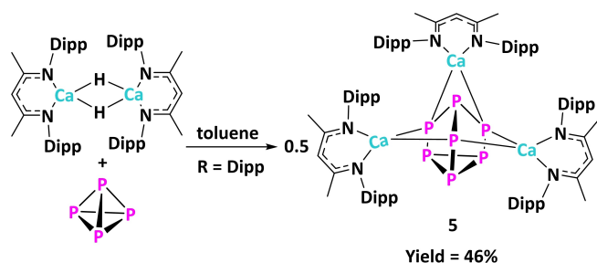
Scheme 5. Synthesis of complex 5.
