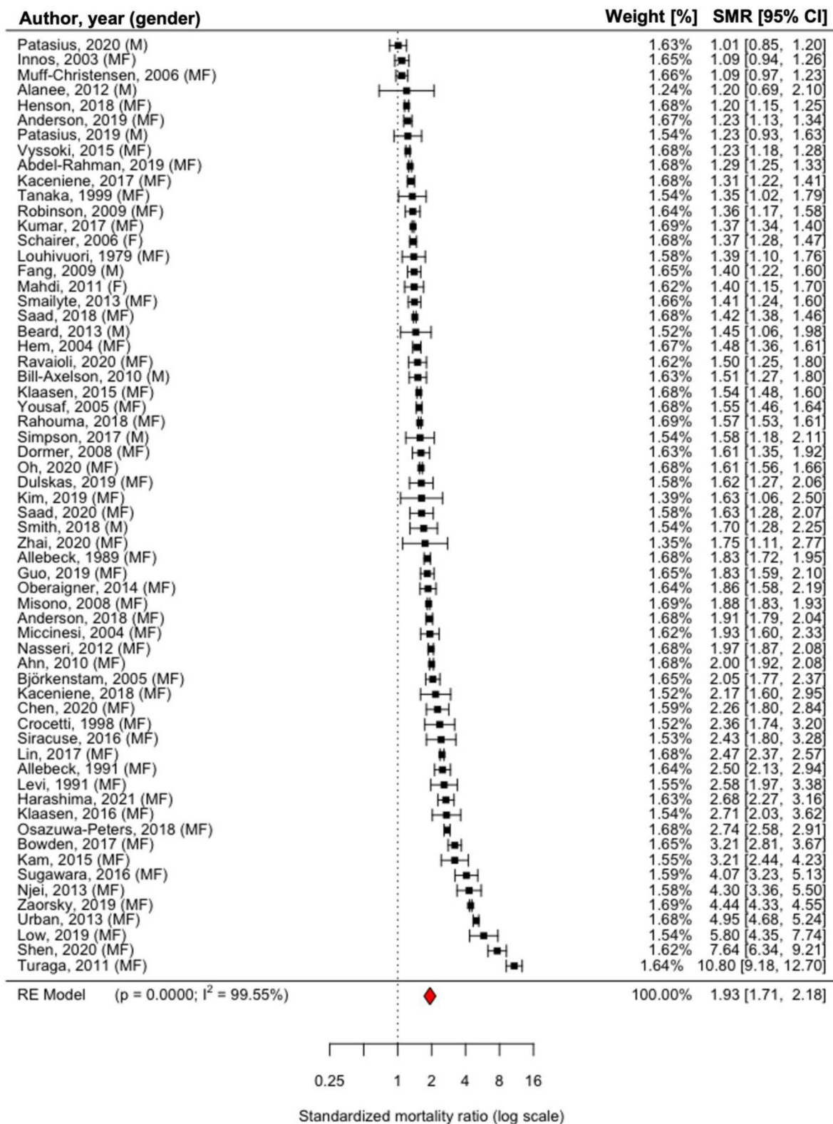
Extended Data Fig. 2 | Forest plot of random effects meta-analysis including 62 cohort studies of suicide in cancer patients extracted from all databases. Studies are listed by magnitude of risk estimate and weighted by their contribution to the summary risk estimate. I^2 = 99.55\% , P -heterogeneity < 0.0001 . Abbreviations: SMR, standardized mortality ratio; CI, confidence interval; MF, men and women combined; M, men only; F, women only; RE, risk estimate. Squares depict SMR point estimates and error bars their corresponding 95% confidence intervals.
