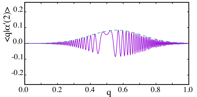
FIG. 4. Countering wave packet spreading. The real (solid purple) and absolute (dashed green) values of \langle q|\alpha'(2)\rangle are shown. Applying the unitary transformation associated with the local linear canonical transformation of the inverse one-step stability matrix undoes wave packet spreading without shifting the position or momentum centroids and generates the second panel from the top of Fig. 3.
