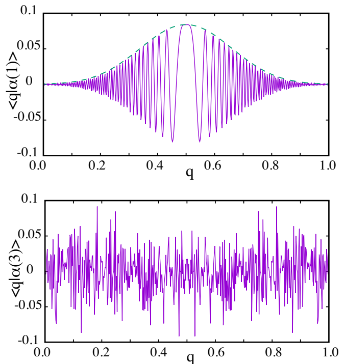
FIG. 2. Quantum chaotic spreading of the kicked rotor initial state |\alpha\rangle . The real (purple solid) and absolute (dashed green) values of the one and three time propagations of the initial state, \langle q | \alpha(1) \rangle (top panel) and \langle q | \alpha(3) \rangle (bottom panel). If uncontrolled the state spreads and rapidly acquires an ergodic looking appearance.
