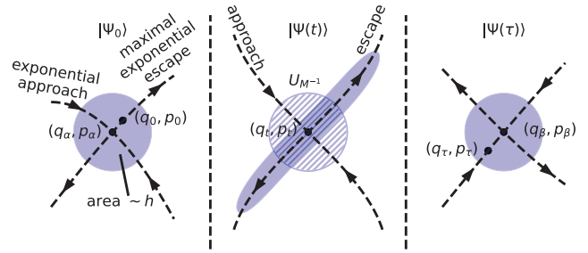
FIG. 1. Schematic of optimal coherent chaotic quantum targeting. The circular zone represents the Wigner transform density of a nearly minimal uncertainty state, which can be slightly shifted (via a unitary operator, U_s ) to be centered on an optimal trajectory starting at (q_0, p_0) . As it propagates the density follows an optimal chaotic trajectory, but is locally spreading, which must be counteracted by contractions, U_{M-1} . At the end, it can be shifted from (q_\tau, p_\tau) to the centroid of the target state (q_\beta, p_\beta) .
