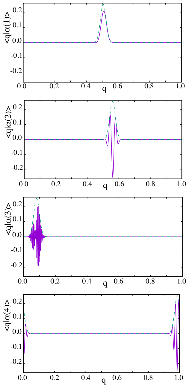
FIG. 3. Quantum guiding along heteroclinic classical paths. The real (solid purple) and absolute (dashed green) values of \langle q|\alpha(t)\rangle are obtained using Eq. (3). At each step the propagated state has a near perfect overlap (not discernible directly from the figure) with a wave packet of the form of Eq. (11) with the time appropriate point of the heteroclinic trajectory in Table I.
