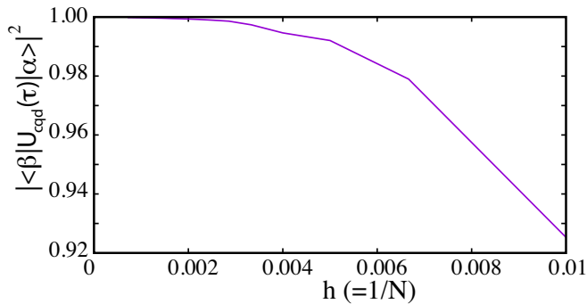
FIG. 5. Fidelity of quantum targeting for the kicked rotor. The squared overlap of the target state with the controlled propagated state, i.e. |\langle \beta | U_{cqd}(\tau = 4) | \alpha(0) \rangle|^2 , see Eq. (3), is plotted versus Planck's constant. As \hbar \rightarrow 0 , the error tends to vanish exponentially. Dimensionalities ranging from N = 100 to 1450 are included.
