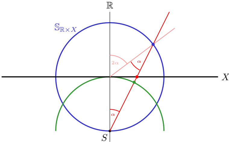
Fig. 2 One-point and disk compactification. The stereographic projection \sigma maps the dot on the circle to the dot on the line, and the map \Theta_X maps the dot on the line to the dot on the half-circle
