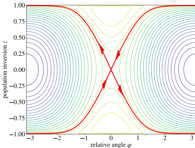
FIG. 3. Reduced phase space structure (z, \varphi) for \Theta_* : contour lines of the Hamiltonian correspond to the classical trajectories. There are three elliptic fixed points and one hyperbolic fixed point whose associated separatrix is highlighted in red. Arrows on the separatrix indicate the stable and unstable manifolds.
