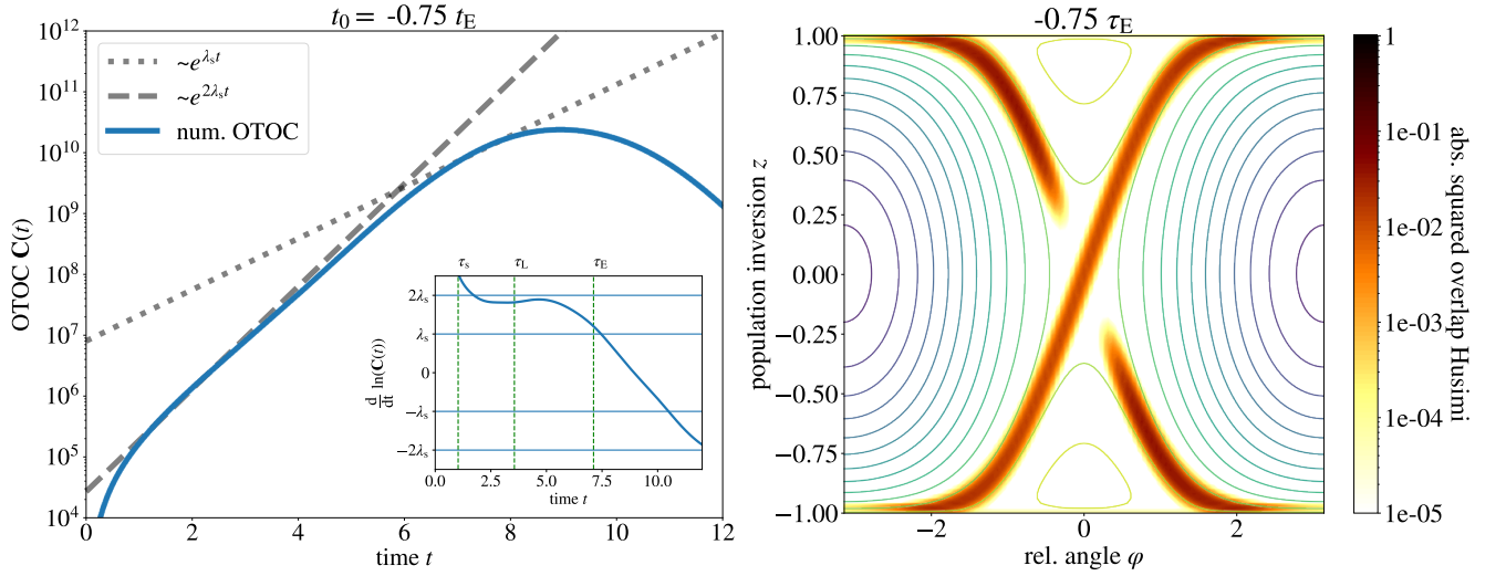
FIG. 7. Left panel: OTOC for a squeezed coherent state for the system parameter \Theta = 1.35 and particle number N = 10^3 . The crossover to \lambda_s vanishes. Right panel: Husimi distribution of the squeezed coherent state. The state is distributed along the stable manifold of the off-phase FP and features tight localization, with a width \sim \hbar_{\text{eff}} , along the unstable manifold.
