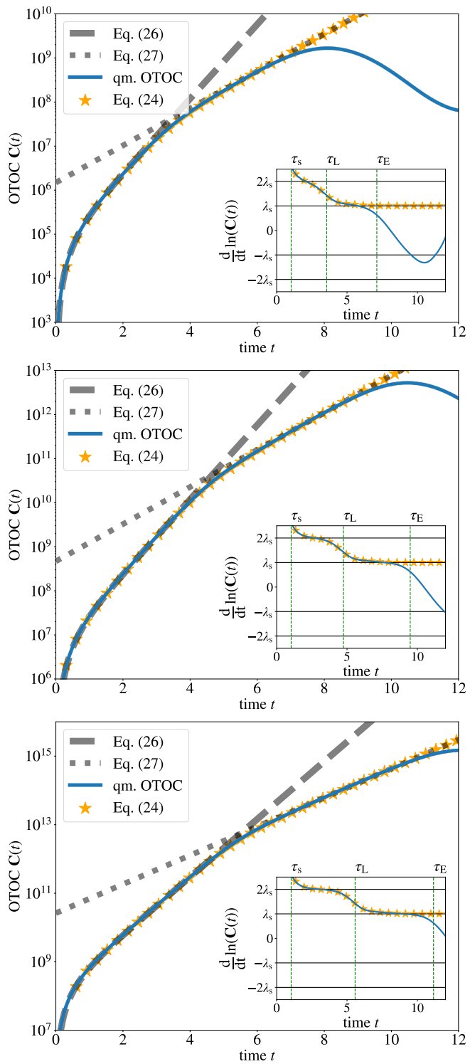
FIG. 4. Top to bottom: OTOC \mathbf{C}(t) for N = 10^3, 10^4, 5 \cdot 10^4 and \Theta = 1.35 ; shaping kink from the 2\lambda_s - \lambda_s transition at \tau_L = \tau_E/2 ; the classical expressions Eq. (26) and Eq. (27) fit tightly the OTOC in each region showing \exp(2\lambda_s t) and \exp(\lambda_s t) exponential growth rates.
