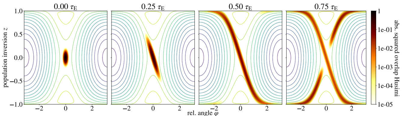
FIG. 5. Time-evolution of the Husimi-distribution for the state |\vec{\xi}\rangle centered at the hyperbolic off-phase FP with N = 10^3 particles. We observe scrambling along the unstable manifold on the separatrix until t \approx \tau_L . The thin lines indicate the classical energy contours to visualize the spreading along the the unstable manifold of the off-phase FP.
