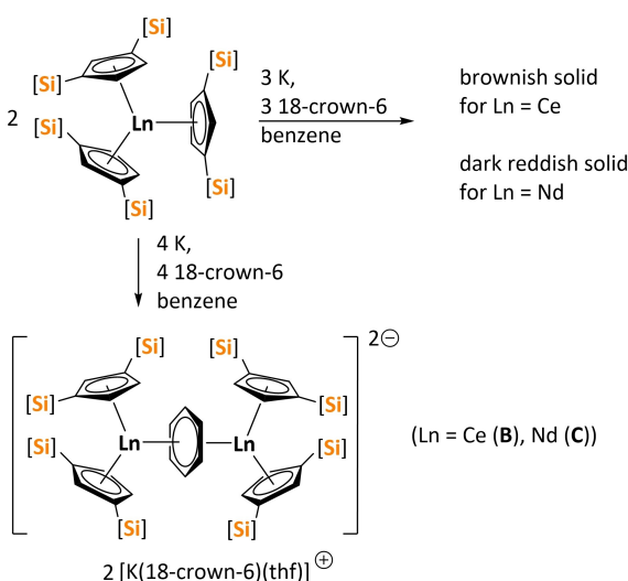
Scheme 3. Investigated reductions of [CeCp'' 3 ] and [NdCp'' 3 ] (analogous towards the synthesis of A ) and synthesis of B (Ln=Ce) and C (Ln=Nd).
