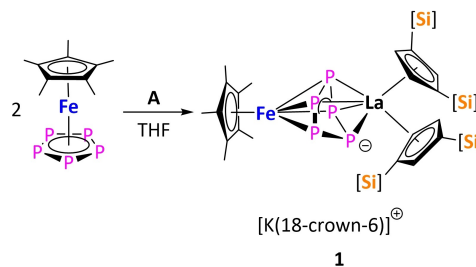
Scheme 2. Synthesis of 1 .
