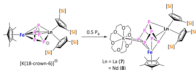
Scheme 6. Synthesis of 7 (Ln = La) and 8 (Ln = Nd) by activation of P 4 .
