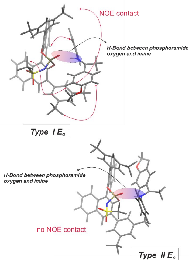
Figure 5: Structures for the oxygen-based H-bonding motif of the binary E-complex: inter-atomic distances obtained from molecular dynamics simulations are consistent with the intense NOE contacts for the Type I E 0 structure (for details and assignment of the substructures to the NOE signals see SI). No NOE contacts were found for the Type II E 0 structure, obtained by rotating the imine leading to the exclusion of structure motif II.
