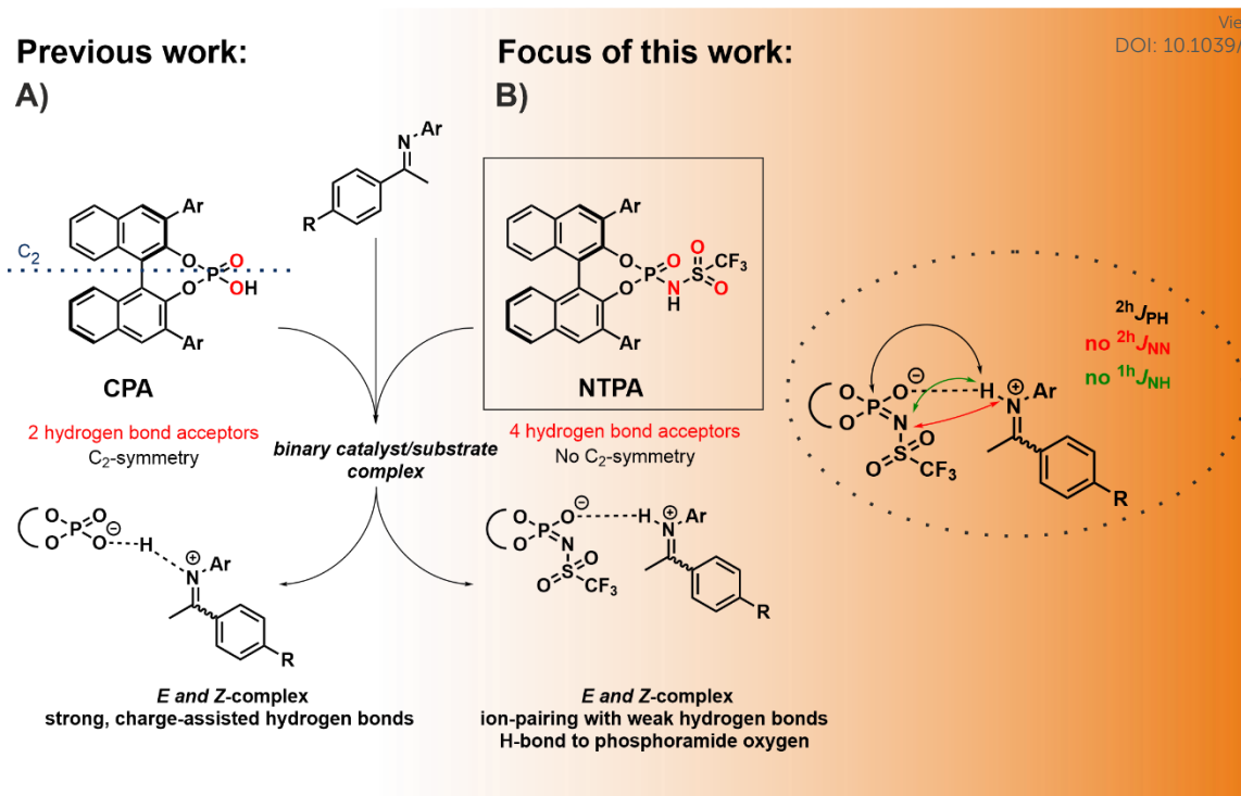
Figure 1: A) Previously binary complexes between CPAs and imines have been studied proving the formation of strong, charge-assisted hydrogen bonds. For the CPA/imine complexes, two different orientations of each imine isomer ( E and Z ) inside the binary complex were detected. B) The focus of this work was a hydrogen bond and a structural analysis of NTPA/imine complexes addressing the influence of increased acidity of the catalyst, multiple hydrogen bond acceptors and the missing C 2 symmetry.
