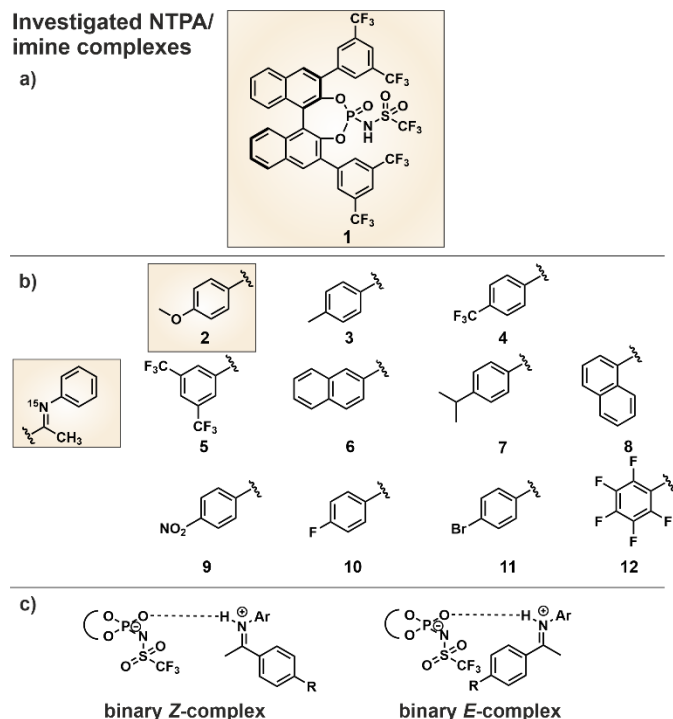
Figure 2: a) NTPA catalyst 1 was selected due to its 3,3'-substituents, which provide the opportunity for ^{19}\text{F} NMR measurements. b) Structures of the imines 2-12 for the hydrogen bond analysis to cover a broad basicity range. Imine 2 was investigated in detail with NTPA 1 to gain structural insights into the binary NTPA/imine complexes. c) The focus of this work was the NMR-spectroscopic investigation of the binary NTPA/imine complexes to clarify which of the several hydrogen bond acceptors is included in the weak hydrogen bond. The imine exists either as E - or Z -isomer.
