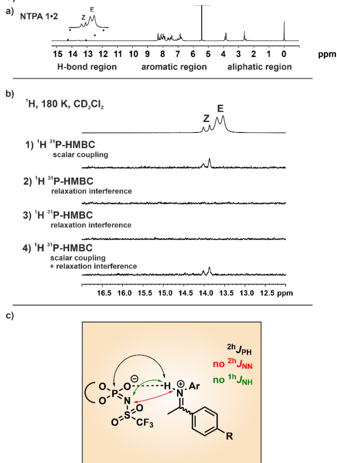
Figure 4: a) ^1\text{H} NMR spectra of the binary complexes between NTPA 1 and imine 2 at 180 K (600 MHz). Generally, the ^1\text{H} NMR spectra can be divided into an H-bond region, an aromatic region, and an aliphatic region. b) ^1\text{H} , ^{31}\text{P} HMBC H-bond section of the NTPA 1/imine 2 complex at 180 K and 600 MHz in \text{CD}_2\text{Cl}_2 . 1) Polarization transfer is mediated only by scalar coupling 2) and 3) Polarization transfer is mediated by ^1\text{H} -CSA and ^1\text{H} ^{31}\text{P} -DD cross relaxation. 4) Polarization transfer is mediated by the sum of scalar coupling and the ^1\text{H} -CSA and ^1\text{H} ^{31}\text{P} -DD cross relaxation. c) binary complex of NTPA 1 and imine 2. ^2\text{H}_\text{PH} coupling was detected in a ^1\text{H} , ^{31}\text{P} HMBC experiment, whereas neither the ^2\text{H}_\text{NN} coupling nor the ^1\text{H}_\text{NH} coupling could be detected in a 1D ^{15}\text{N} or 2D ^1\text{H} , ^{15}\text{N} -HSQC spectrum.
