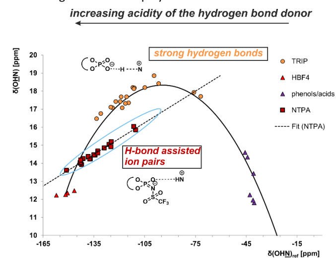
Figure 3: Plot of \delta(\text{OHN})_{\text{ref}} against \delta(\text{OHN}) for various binary NTPA 1 /imine and CPA/imine complexes. The ^{15}\text{N} chemical shifts are referenced by \delta(\text{OHN})_{\text{ref}} = \delta(\text{OHN})_{\text{obs}} - 340.8 ppm. 340.8 ppm is the chemical shift of the free imine showing the strongest hydrogen bond in the previous work. Data points of phenols/carboxylic acids, tetrafluoroboric acid and the CPA TRIP are from previous studies (see SI). Binary E - and Z -complexes of NTPA 1 and imines 2-12 are depicted in red rectangles and show a deviation from the correlation curve. This is an indication for a double-well potential, which means the proton is either located at the proton acceptor or donor.
