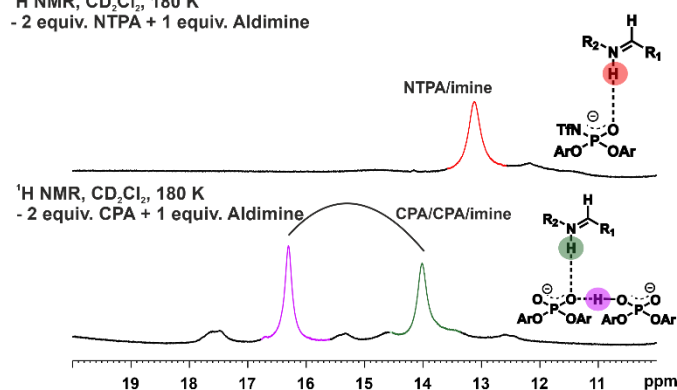
Figure 6: Low-temperature NMR at 180 K was used to investigate the presence of dimers in a 2:1 ratio of catalyst to imine. In the samples with a 2:1 ratio of NTPA to imine, no dimeric formation was identified. However, when employing a 2:1 ratio with CPA to imine, dimer formation became evident in the 1 H NMR spectrum.
