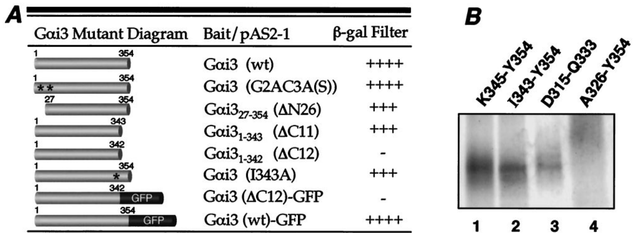
Fig. 5. Calnuc interacts with the C-terminal \alpha 5 -helix of Gai3. (A) Two-hybrid assays. Gai3 mutants were subcloned into the pAS2–1 bait vector, and calnuc was constructed in the pACT2 prey vector. The \beta -galactosidase filter assay was performed on (Leu - , Trp - ) plates, and color was scored after 2 h. (–, negative; +, weak; ++, intermediate; +++, strong; +++++, very strong). Gai3 mutants in which N-terminal sites for both myristoylation and palmitoylation were mutated [G2AC3A(S)] or the first 26 amino acids were truncated (ΔN26) bind to calnuc as strongly as wild-type (wt) Gai3. Similarly, truncation of the last 11 C-terminal amino acids (Gai3 ΔC11) does not reduce Gai3 binding to calnuc whereas the interaction is completely abolished by deletion of the last 12 C-terminal amino acids (Gai3 ΔC12). However, Gai3 (I343A) still strongly binds to calnuc. Addition of GFP to the Gai3 mutant with the C-terminal 12 amino acids deleted (Gai3 ΔC12-GFP) does not restore binding to calnuc. Full length Gai3 (wt)-GFP shows strong interaction with calnuc. Reproducible results were obtained in three separate experiments. (B) Peptide competition assays. 2 mM of each of four synthetic peptides and in vitro translated [ 35 S]Gai3 were incubated with calnuc-Sepharose 4B in the presence of 15 mM Mg 2+ /2 mM Ca 2+ as described in Fig. 2A, followed by SDS/PAGE and autoradiographic analysis. The peptides K345–Y354 (lane 1), I343–Y354 (lane 2), and D315–Q333 (lane 3) are not able to compete [ 35 S]Gai3 binding to calnuc whereas peptide A326–Y354 (lane 4) completely inhibits calnuc–Gai3 interaction.
