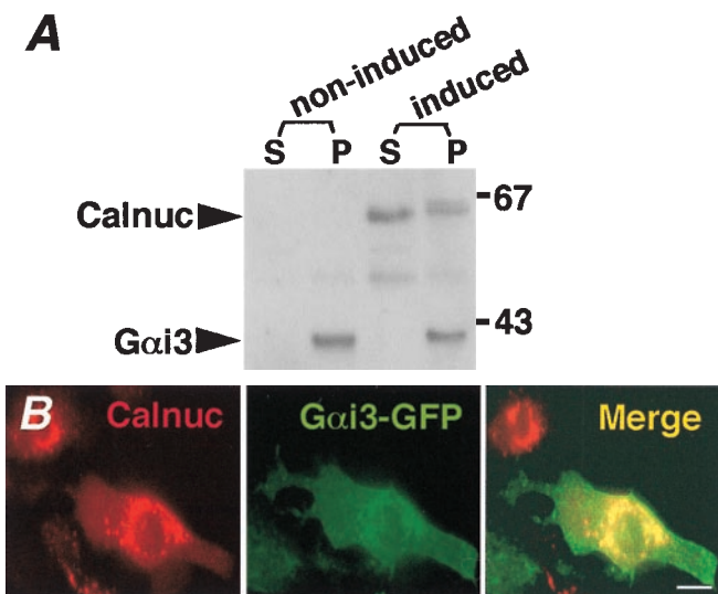
Fig. 3. Localization of Calnuc and G\alpha i3 . (A) Expression of G\alpha i3 in non-induced and induced ( 10 \mu\text{M} ponasterone A for 48 h) EcR-CHO-Calnuc cells stably overexpressing calnuc. Cytosolic ( 100,000 \times g supernatant) and membrane ( 100,000 \times g pellet) fractions were prepared and immunoblotted with anti-calnuc IgG and affinity-purified anti- G\alpha i3 IgG (EC). The ratio of the cytosolic (S) and membrane-associated (P) pools of overexpressed calnuc is \approx 60:40 . The cytosolic pool shows a faster mobility than that of the membrane pool, which consists of two bands. Overexpression of calnuc does not significantly affect the level and distribution of endogenous G\alpha i3 , which is found exclusively in the membrane fraction (P). However, the mobility of G\alpha i3 is reduced slightly. (B) Immunofluorescence. EcR-CHO-Calnuc cells were transiently transfected with G\alpha i3 -GFP cDNA, followed by induction with 10 \mu\text{M} ponasterone A for 48 h. To maintain intracellular divalent ion concentration, cells were treated with 10 \mu\text{M} ionomycin/ 2 \text{ mM} \text{Ca}^{2+} / 15 \text{ mM} \text{Mg}^{2+} , followed by fixation in 2% formaldehyde and incubation with anti-calnuc IgG and Texas Red-conjugated donkey anti-rabbit F(ab) _2 . Overexpressed calnuc (Left) was detected in the Golgi region and in the cytoplasm. G\alpha i3 -GFP (Middle) was found on the plasma membrane as well as in the Golgi region. The merged images (Right) indicate that the distribution of calnuc and G\alpha i3 partially overlap mainly in the Golgi region. (Bar = 10 \mu\text{m} .)
