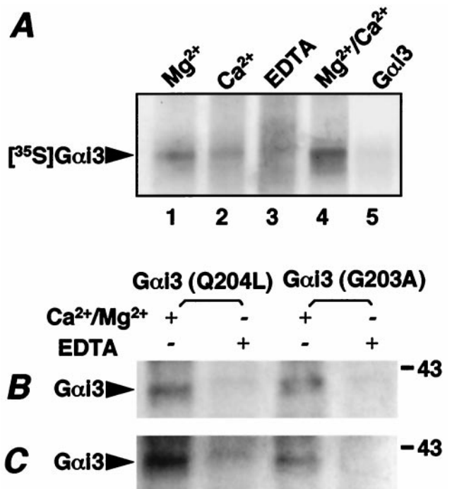
Fig. 2. Calnuc specifically interacts with both activated and inactivated Gai3 in vivo , and the interaction is Ca^{2+} / Mg^{2+} -dependent. (A) Pull-down assays. In vitro translated [ ^{35} S] Gai3 was incubated with calnuc-Sepharose 4B at 4°C for 1 h in the presence of 15 mM Mg^{2+} (lane 1), 2 mM Ca^{2+} (lane 2), 15 mM Mg^{2+} + 2 mM Ca^{2+} (lanes 4 and 5), or 5 mM EDTA (lane 3), followed by extensive washing, SDS/PAGE separation, and autoradiographic analysis. Calnuc interacts with [ ^{35} S] Gai3 in the presence of Mg^{2+} , Ca^{2+} , or both, but weak interaction is observed in the presence of Ca^{2+} alone. Binding is abolished by 5 mM EDTA as well as excess unlabeled Gai3 (lane 5). (B) coIP of Gai3 and calnuc. NIH 3T3 cells overexpressing Gai3 (Q204L) (activated) and Gai3 (G203A) (inactivated) were lysed with 0.5% TX-100 at 4°C for 30 min in the presence of 2 mM Ca^{2+} /15 mM Mg^{2+} or 5 mM EDTA. coIP was performed on the cell lysates with anti-calnuc IgG in the presence of 1 M NDSB-195 and protein A beads, as described in Materials and Methods , followed by immunoblotting with anti- Gai3 IgG. Calnuc interacts with both activated and inactivated Gai3 in the presence (+) but not in the absence (–) of 2 mM Ca^{2+} /15 mM Mg^{2+} , suggesting that the interaction between calnuc and Gai3 is Ca^{2+} / Mg^{2+} -dependent but does not depend on the state of activation of Gai3 . (C) Crosslinking of calnuc and Gai3 . NIH 3T3 cells overexpressing Gai3 (Q204L) and Gai3 (G203A) cells were treated with 10 \mu M ionomycin plus either 2 mM Ca^{2+} /15 mM Mg^{2+} or 5 mM EDTA. Crosslinking was carried out by using the membrane permeant crosslinker dithiobis (succinimidylpropionate) (2 mM), followed by lysis with 1% TX-100 and immunoprecipitation with anti-calnuc IgG as above. Similar results to those in B were obtained. Both coIP and crosslinking experiments were repeated four times.
