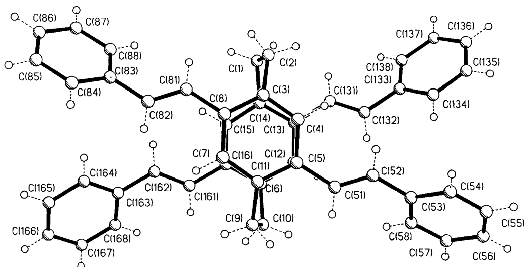
Figure 2. Molecular structure of 4,7,12,15-tetrastyril[2.2]paracyclophane ( 7a ). Selected bond lengths [pm]: C(1)–C(2) 158.4(3), C(2)–C(3) 151.8(3), C(3)–C(4) 138.7(4), C(3)–C(8) 140.4(4), C(4)–C(5) 139.9(3), C(8)–C(81) 147.0(4), C(81)–C(82) 131.6(4), C(82)–C(83) 147.3(4); bond angles [°]: C(1)–C(2)–C(3) 111.8(2), C(2)–C(3)–C(8) 123.0(2), C(4)–C(3)–C(8) 117.6(2), C(3)–C(4)–C(5) 123.0(2), C(4)–C(5)–C(51) 120.5(2), C(10)–C(11)–C(16) 122.2(2), C(5)–C(51)–C(52) 127.1(2), C(52)–C(53)–C(54) 121.0(3); dihedral angles [°]: C(3)–C(2)–C(1)–C(14) 22.3, C(4)–C(5)–C(51)–C(52) 26.6, C(5)–C(51)–C(52)–C(53) 9.7, C(51)–C(52)–C(53)–C(54) 22.1; bending of para -bridged benzene rings: angle between axis C(2)–C(3) and plane C(4)–C(3)–C(8) 12.5°, angle between plane C(4)–C(3)–C(8) and plane C(4)–C(5)–C(7)–C(8) 12.8°
