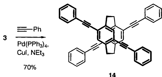
Figure 2. Molecular structure of 4,7,12,15-tetrastyril[2.2]paracyclophane ( 7a ). Selected bond lengths [pm]: C(1)–C(2) 158.4(3), C(2)–C(3) 151.8(3), C(3)–C(4) 138.7(4), C(3)–C(8) 140.4(4), C(4)–C(5) 139.9(3), C(8)–C(81) 147.0(4), C(81)–C(82) 131.6(4), C(82)–C(83) 147.3(4); bond angles [°]: C(1)–C(2)–C(3) 111.8(2), C(2)–C(3)–C(8) 123.0(2), C(4)–C(3)–C(8) 117.6(2), C(3)–C(4)–C(5) 123.0(2), C(4)–C(5)–C(51) 120.5(2), C(10)–C(11)–C(16) 122.2(2), C(5)–C(51)–C(52) 127.1(2), C(52)–C(53)–C(54) 121.0(3); dihedral angles [°]: C(3)–C(2)–C(1)–C(14) 22.3, C(4)–C(5)–C(51)–C(52) 26.6, C(5)–C(51)–C(52)–C(53) 9.7, C(51)–C(52)–C(53)–C(54) 22.1; bending of para -bridged benzene rings: angle between axis C(2)–C(3) and plane C(4)–C(3)–C(8) 12.5°, angle between plane C(4)–C(3)–C(8) and plane C(4)–C(5)–C(7)–C(8) 12.8°
