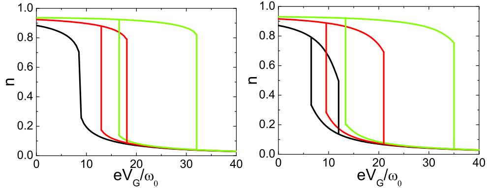
Figure 2. (Color) Bistable behavior of the level population n in the self-consistent Hartree approximation (left) and second approximation (right) as a function of gate voltage for different electron-vibron interaction strength \lambda = 3\omega_0 (black), \lambda = 4\omega_0 (red), \lambda = 5\omega_0 (green), the other parameters are \Gamma = 5\omega_0 , T = 0.25\omega_0 , \eta = 0 and V_B = 0 .
