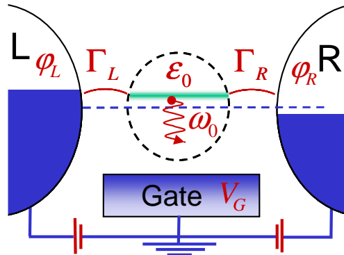
Figure 1. (Color) Schematic representation of a single-level model system interacting with a vibronic mode and coupled to left and right leads.
