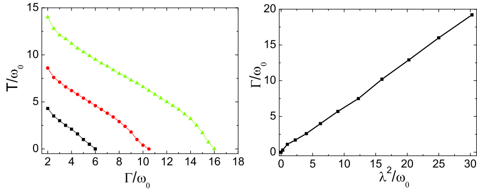
Figure 5. (Color) "Phase diagram" depicting the boundaries between parameter regimes of bistable memory (below the threshold lines) and single-valued states (above threshold). Left panel: \Gamma - T parameter plane at different electron-vibron interaction strength \lambda = 3\omega_0 (black), \lambda = 4\omega_0 (red), \lambda = 5\omega_0 (green); right panel: \lambda - \Gamma parameter plane for T = 0.25\omega_0 .
