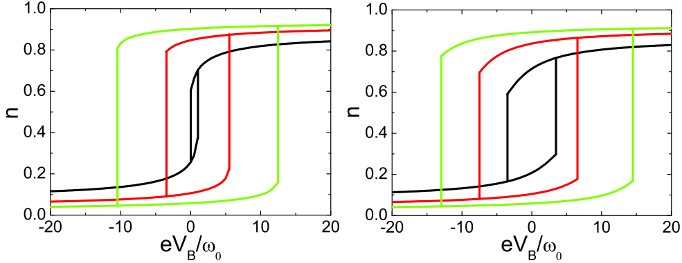
Figure 3. (Color) Level population n in the self-consistent Hartree approximation (left) and the second approximation (right) as a function of normalized bias voltage for different electron-vibron interaction strength \lambda = 3\omega_0 (black), \lambda = 4\omega_0 (red), \lambda = 5\omega_0 (green), the other parameters are \Gamma = 5\omega_0 , T = 0.25\omega_0 , \eta = 0 and V_G = \frac{\lambda^2}{\omega_0} .
